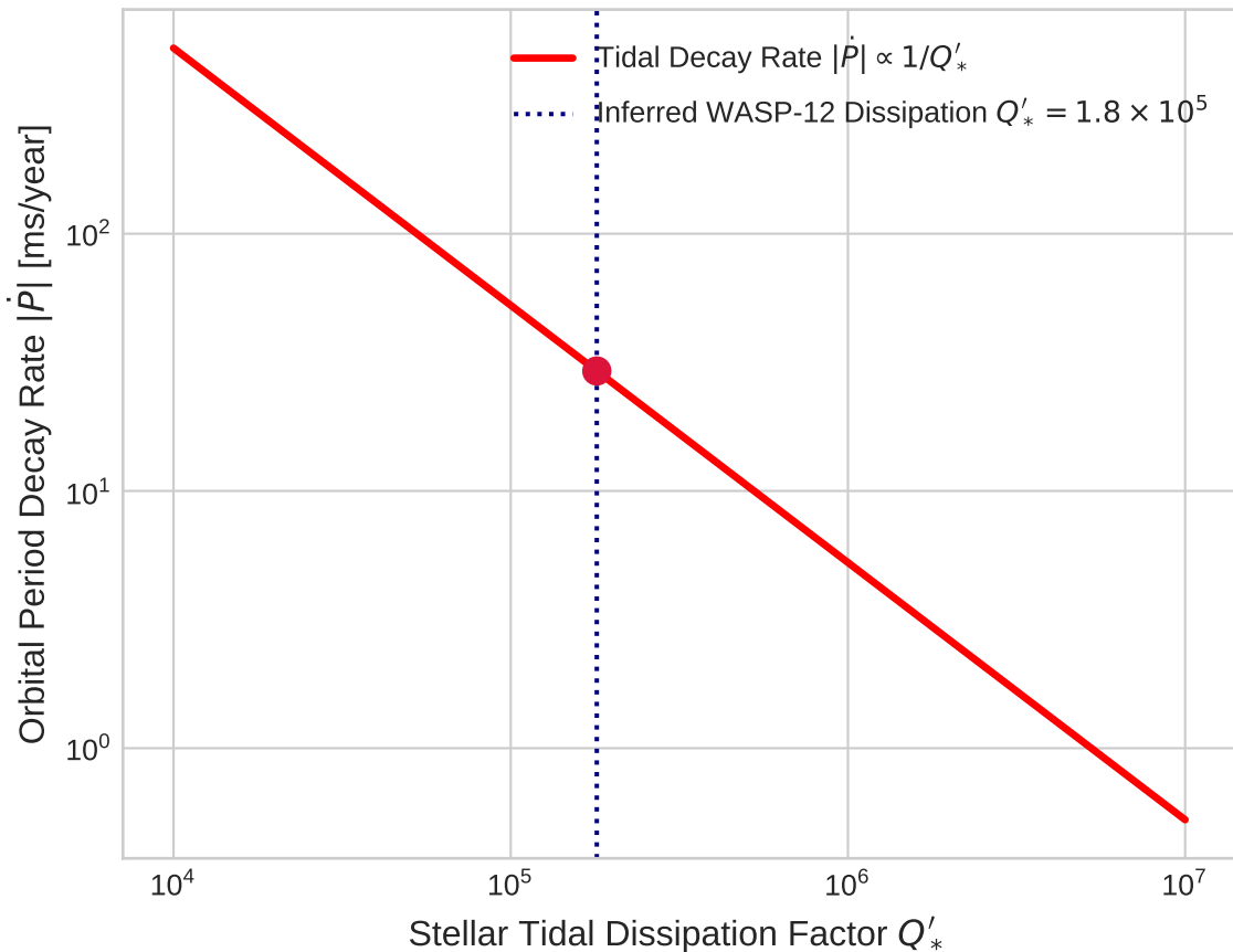
Model Choice: Decay Rate vs Stellar Q'_*
