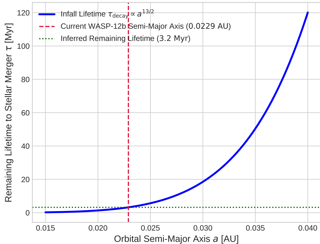
Model Choice: Orbital Lifetime Scaling
