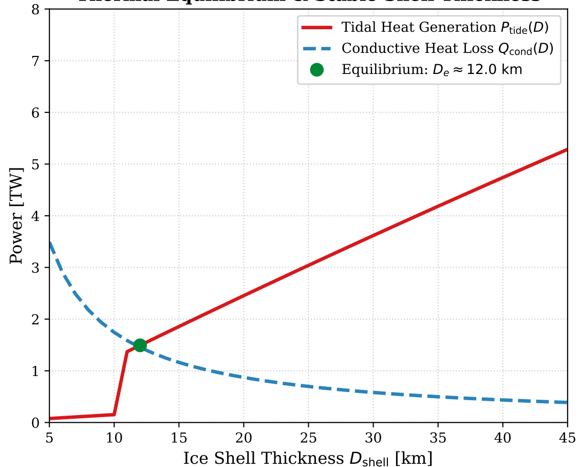
Thermal Equilibrium & Stable Shell Thickness
