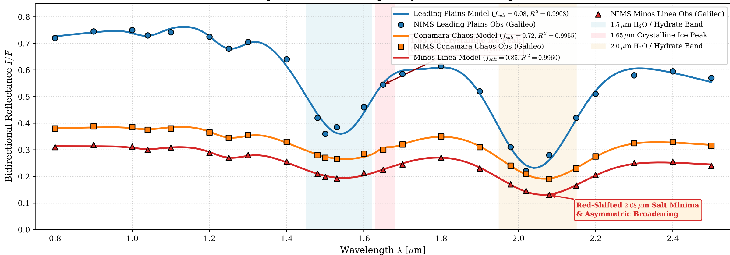
(a) Galileo NIMS Reflectance Spectra vs First-Principles Hydrated Salt Mixing Model (McCord et al. 1998)
