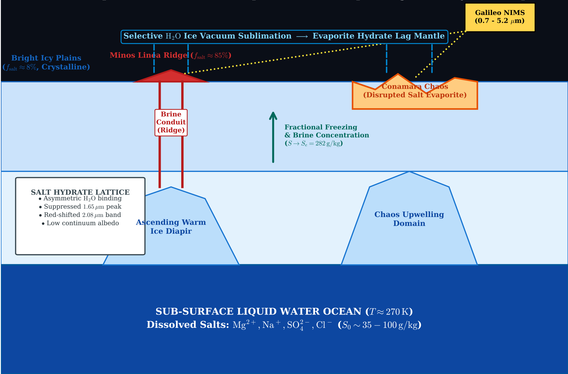
Figure 3: First-Principles Architecture of Europa Ocean Brine Upwelling & Salt Hydration Spectroscopy
