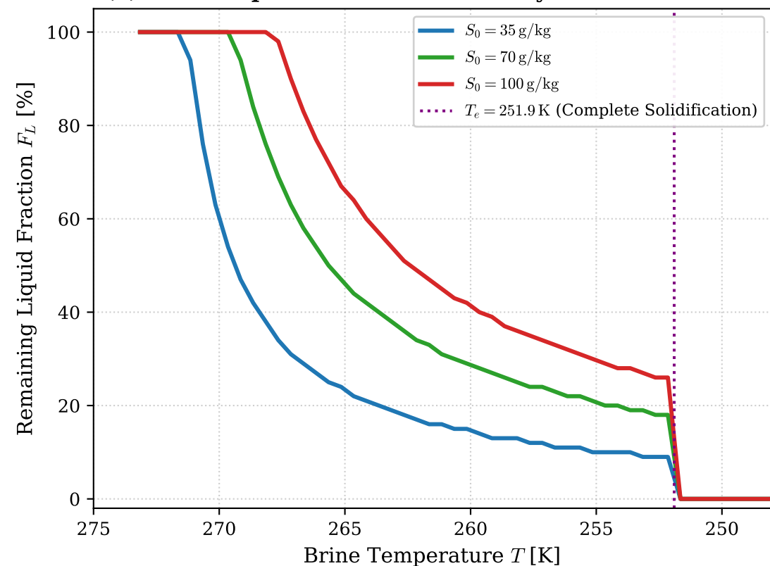
(b) Brine Expulsion & Fractional Crystallization Curve
