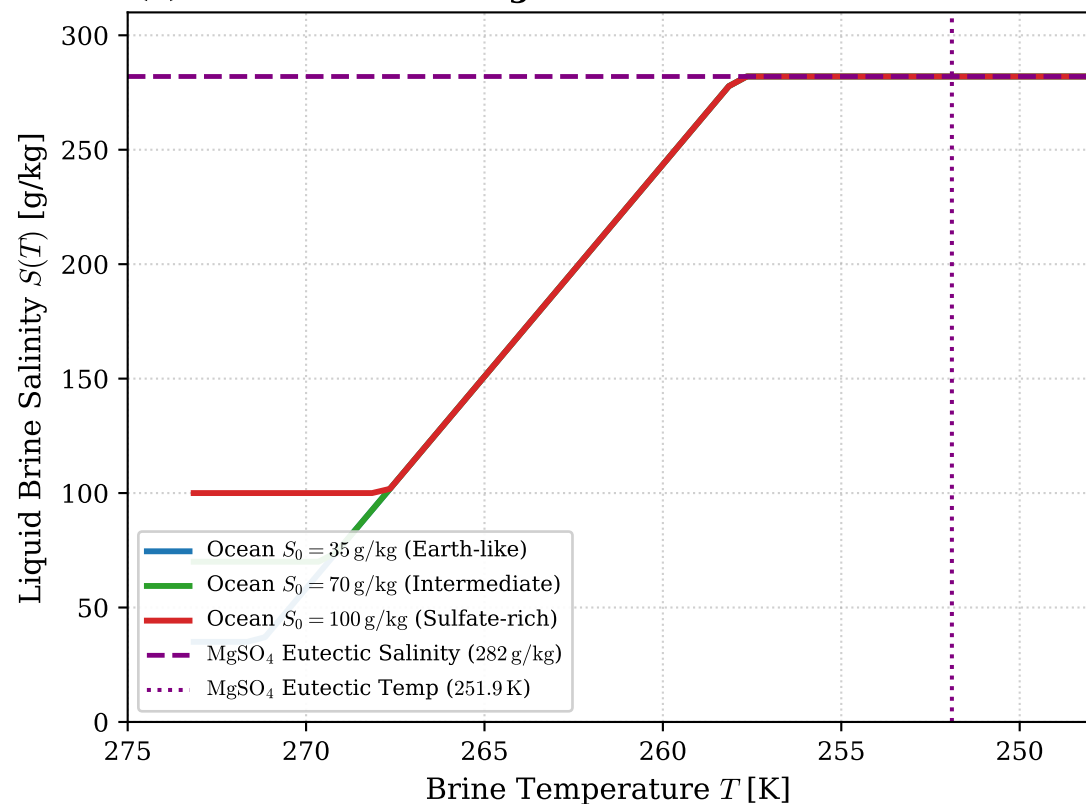
(a) Fractional Freezing & Eutectic Brine Concentration
