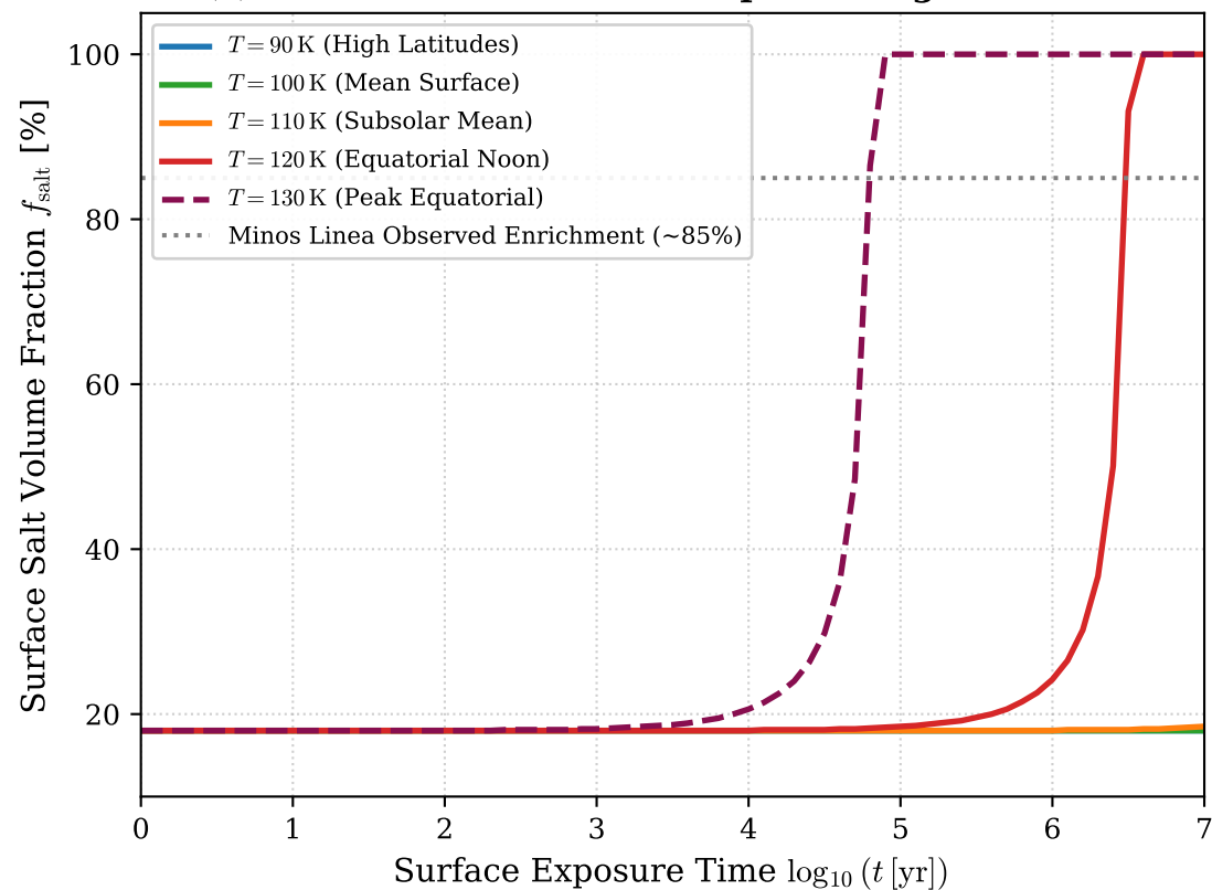
(c) Vacuum Sublimation Evaporite Lag Formation
