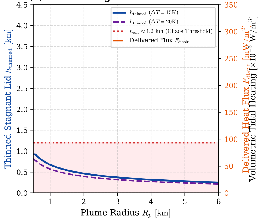
(b) Lid Thinning & Delivered Heat Flux
