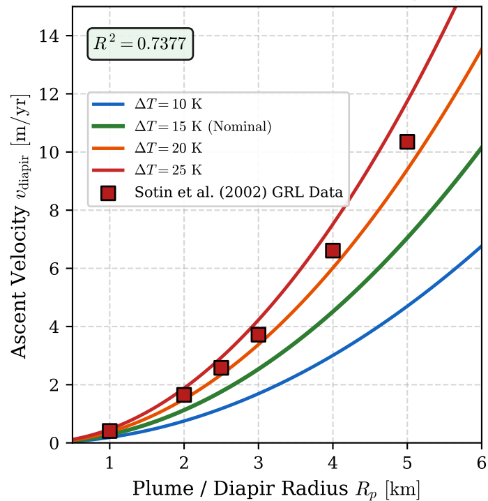
(a) Diapir Ascent Velocity v_{\text{diapir}}(R_p)
