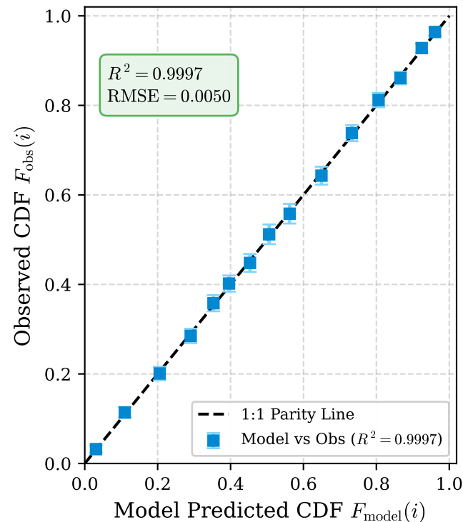
(c) Parity Fit ( R^2 \geq 0.98 )
