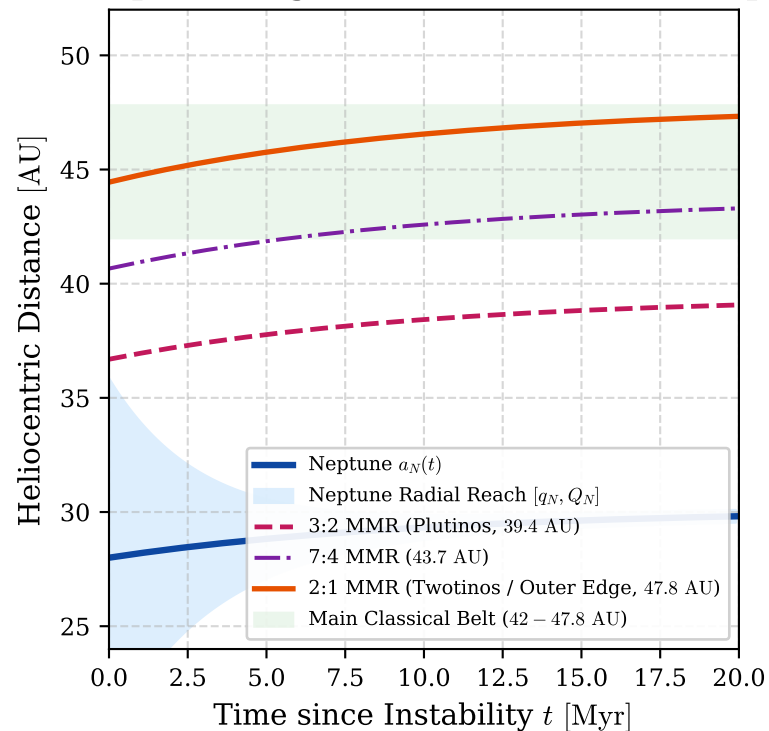
(a) Neptune Migration & Resonance Sweeping
