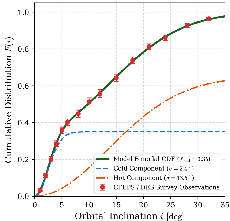
(b) Classical Kuiper Belt Inclination CDF
