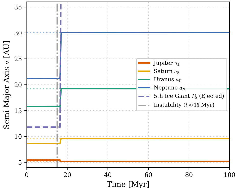
(a) 5-Planet Jumping-Jupiter Orbital Migration
