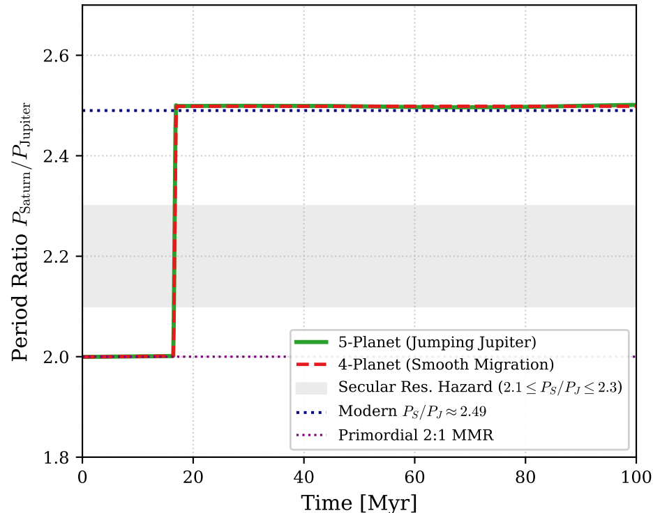
(b) Jumping Period Ratio vs Smooth Sweep
