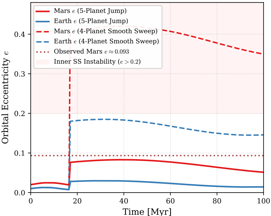
(c) Terrestrial Planet Secular Eccentricity
