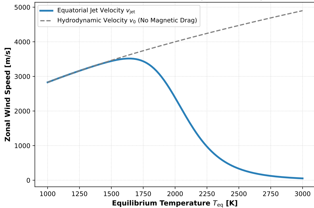
Zonal Wind Deceleration by Lorentz Drag
