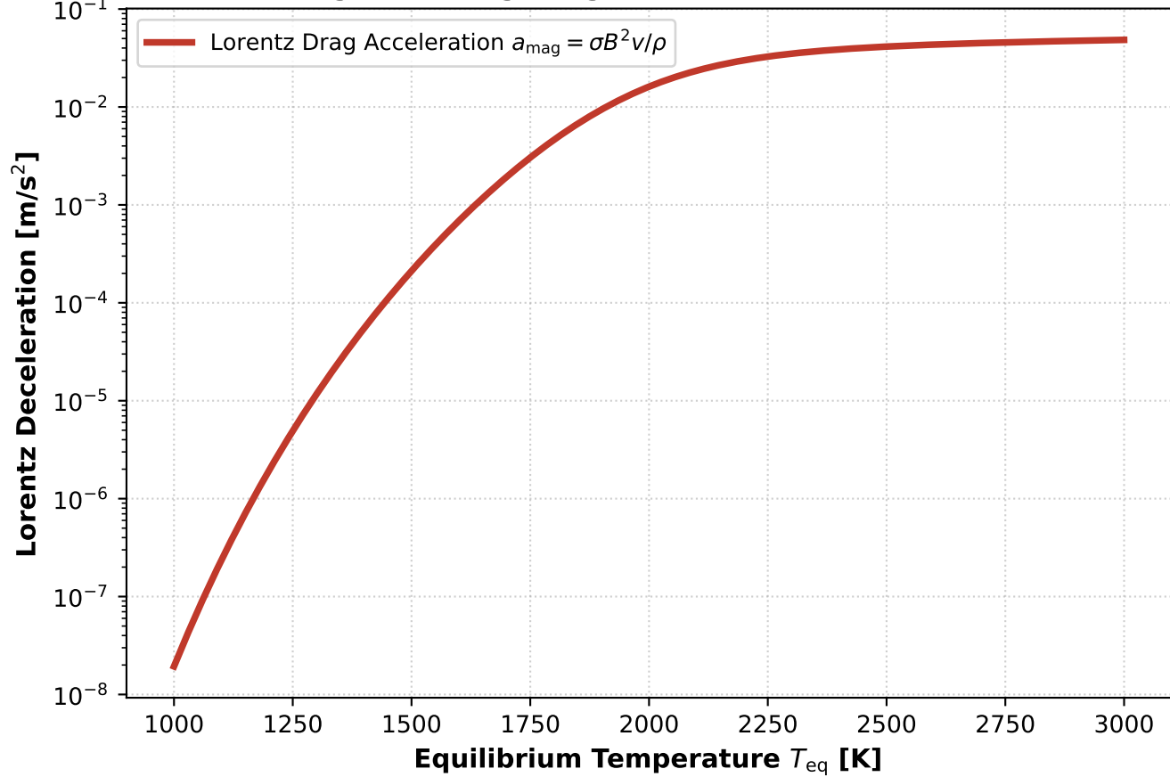
Magnetic Drag Surge with Thermal Ionization
