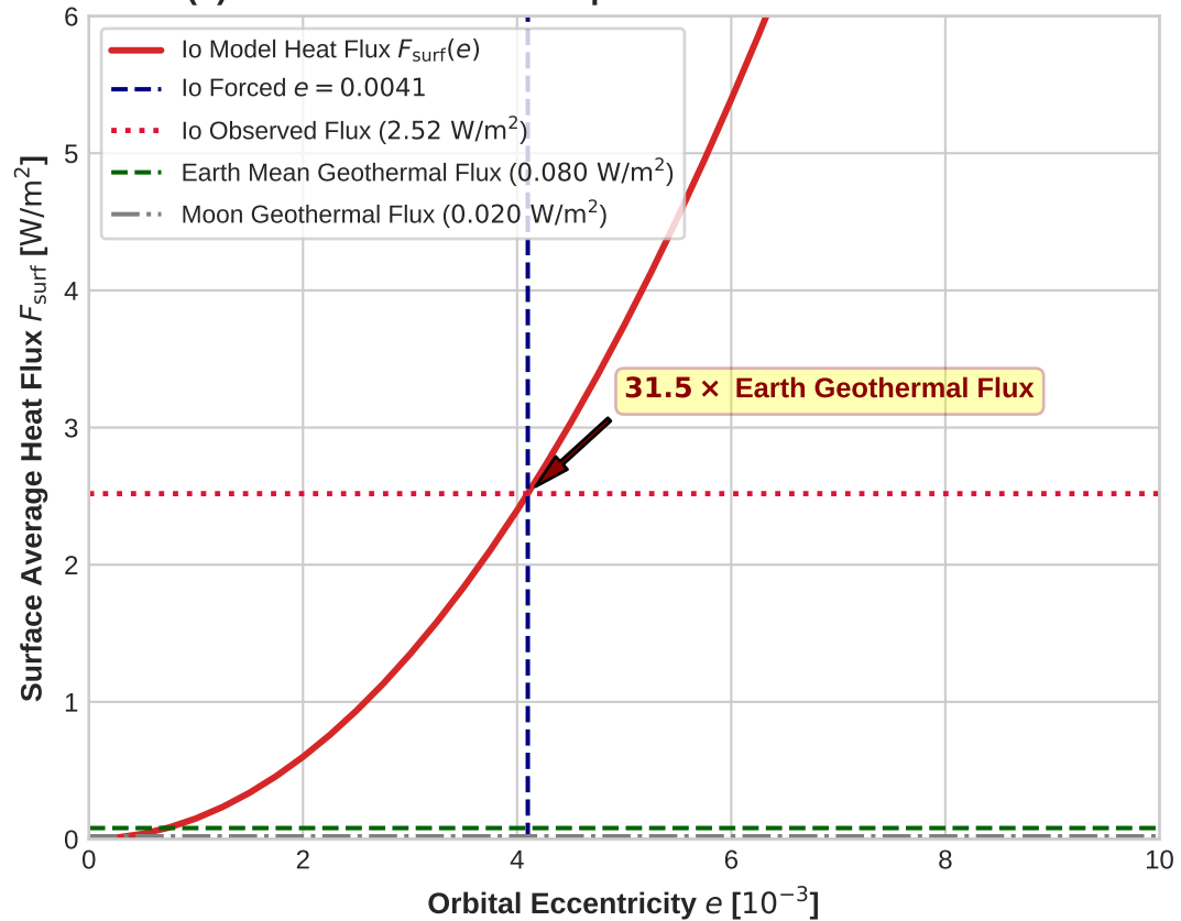
(b) Surface Heat Flux Comparison with Terrestrial Bodies
