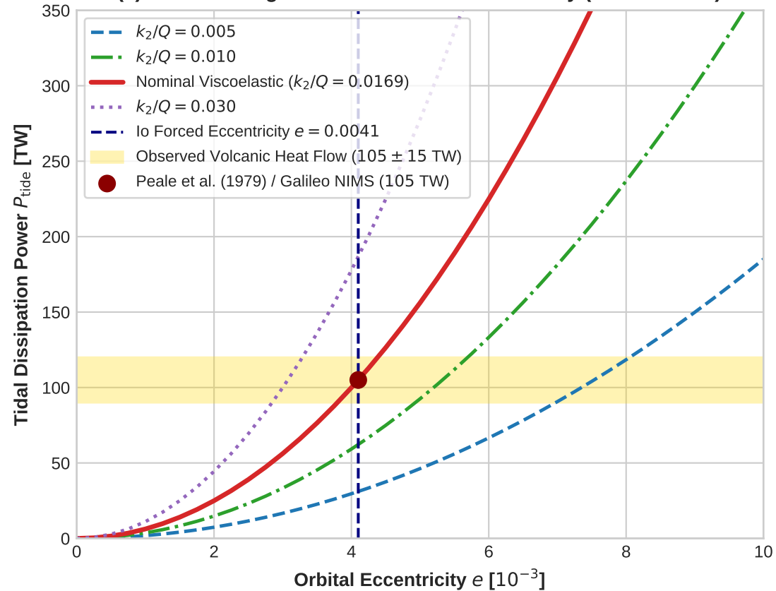
(a) Tidal Heating Power vs. Forced Eccentricity ( R^2 = 0.9999 )
