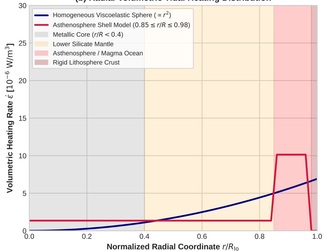
(b) Radial Volumetric Tidal Heating Distribution
