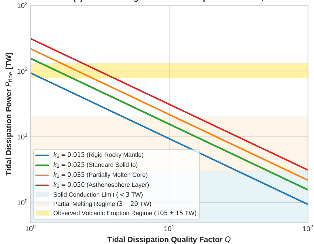
(a) Tidal Heating Power vs. Dissipation Factor Q
