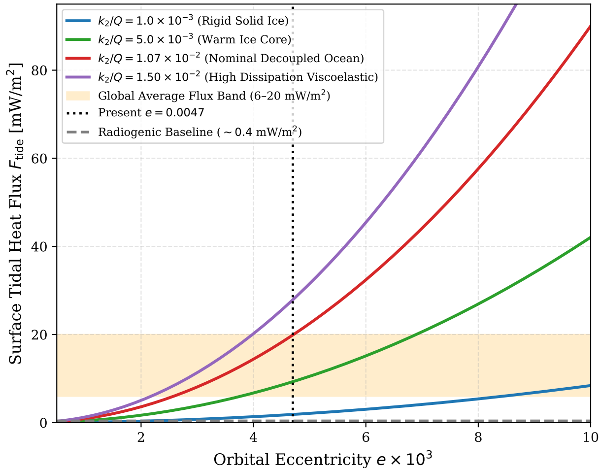
Surface-Averaged Tidal Heat Flux vs. Eccentricity
