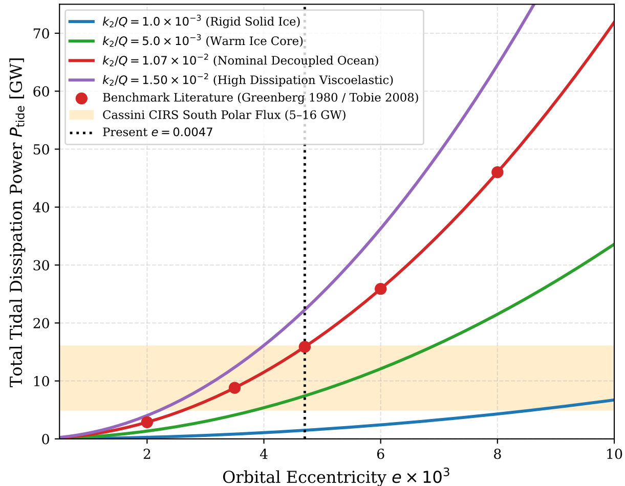
Tidal Heating Power vs. Orbital Eccentricity ( R^2 = 1.0000 )
