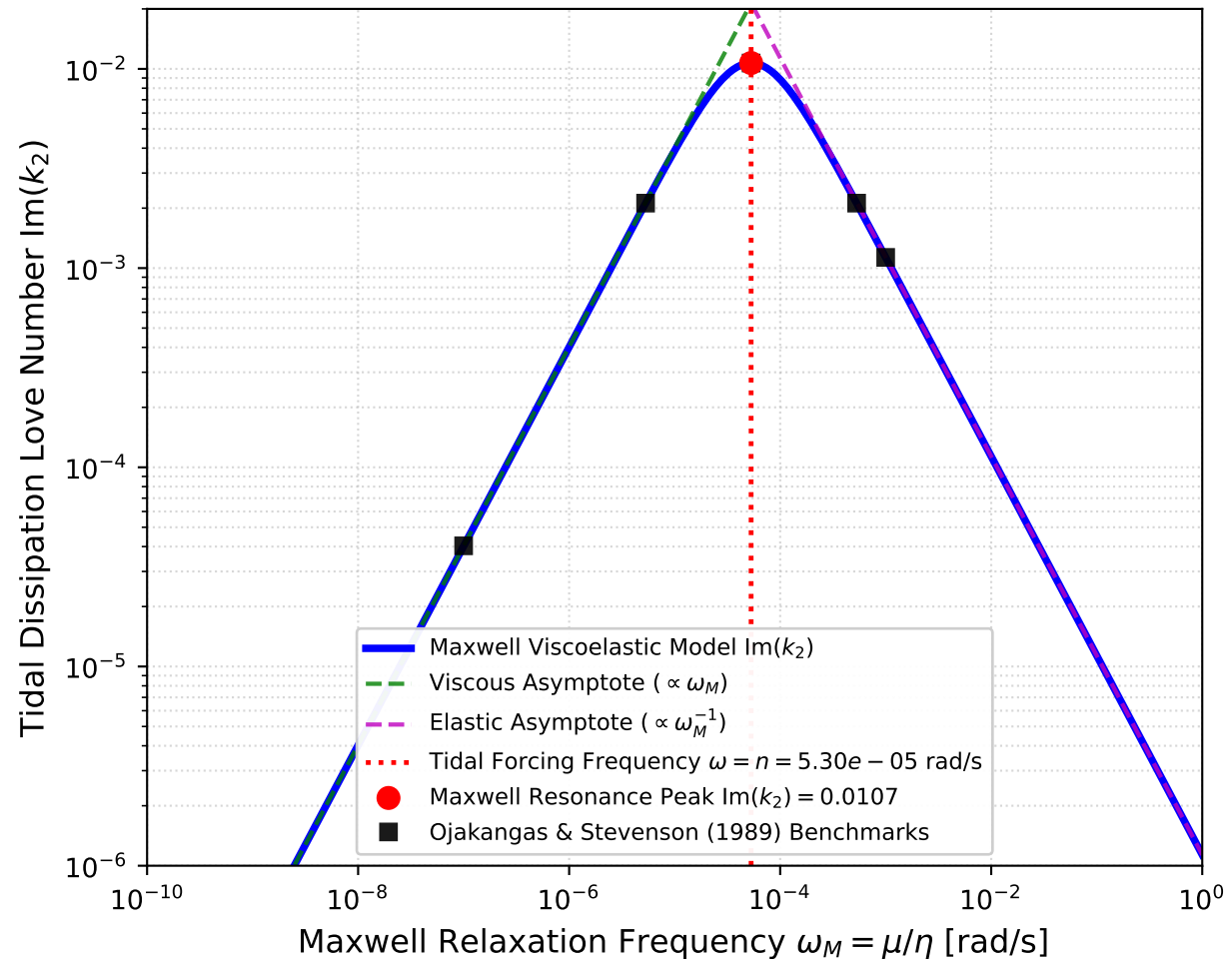
(a) Dissipation Factor \text{Im}(k_2) vs. Maxwell Frequency \omega_M
