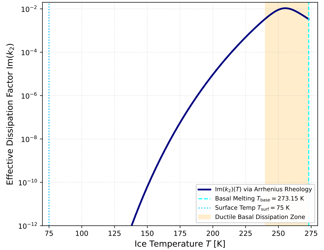
(b) Temperature Activation of Viscoelastic Dissipation
