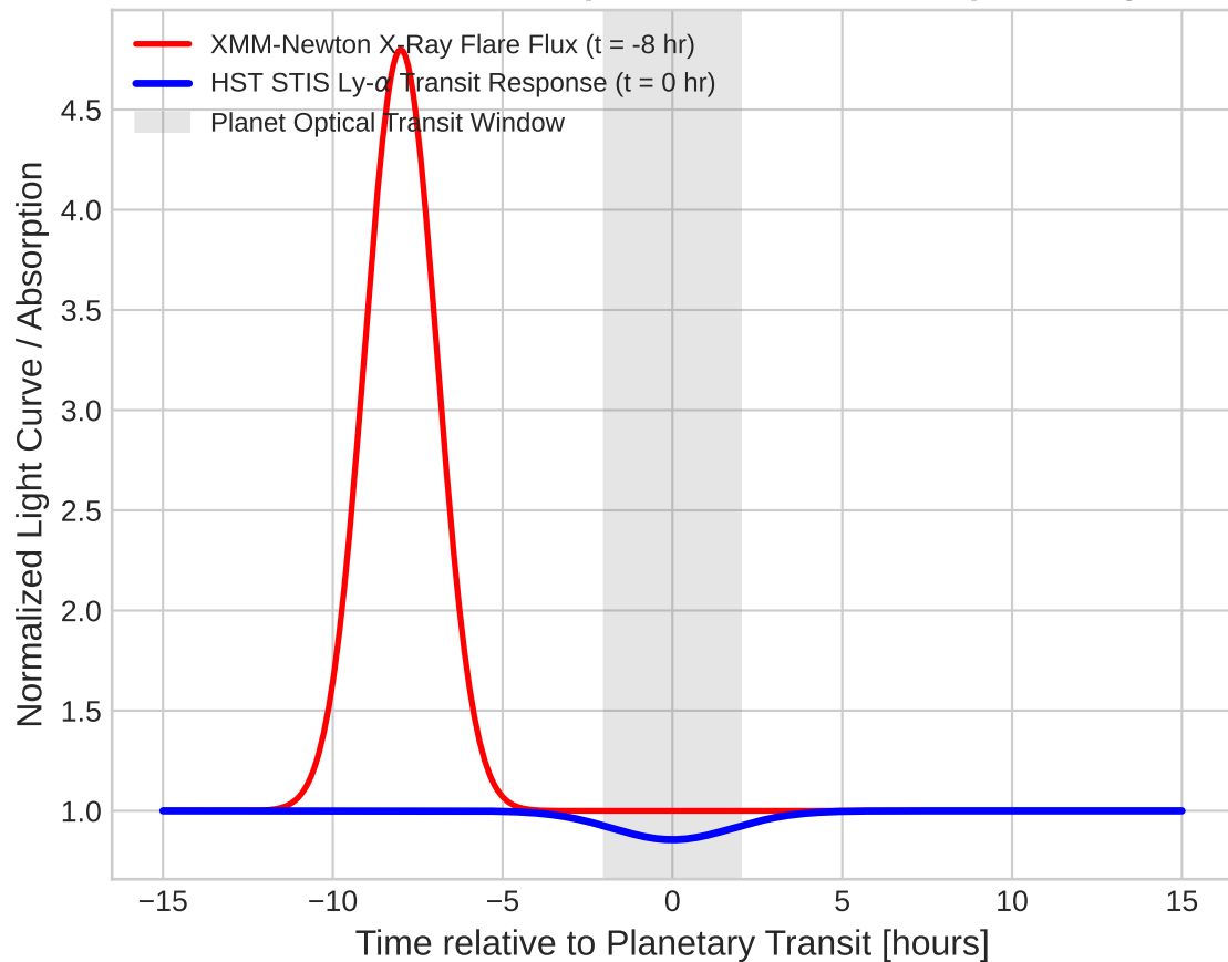
XMM-Newton Flare Spike & HST STIS Temporal Lag
