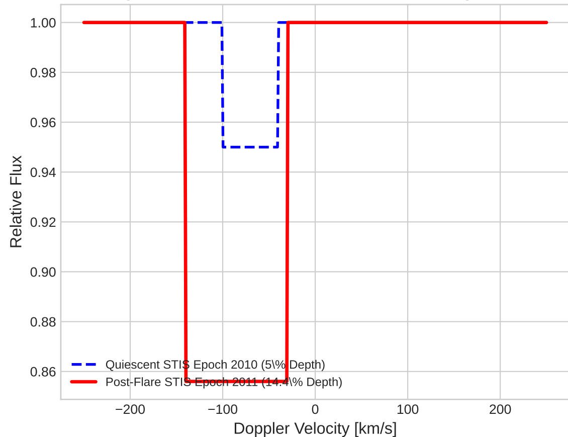
Spectral Line Profile: Quiescent vs Flare Epochs
