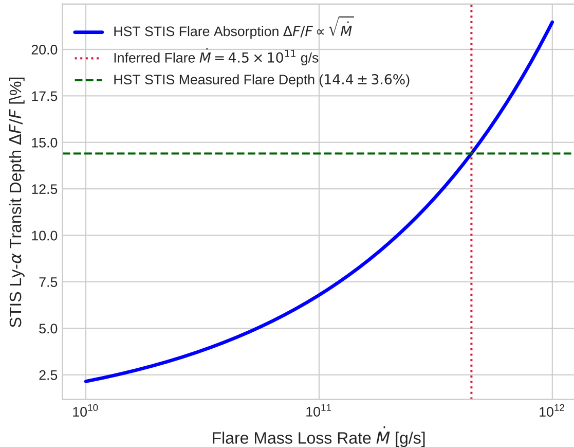
Model Choice: Flare Absorption Sensitivity
