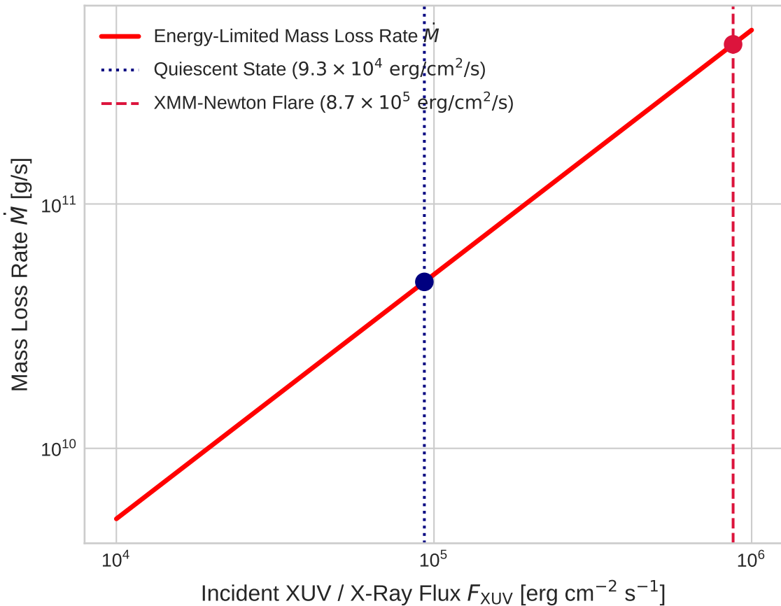
Model Choice: Quiescent vs Flare Mass Loss
