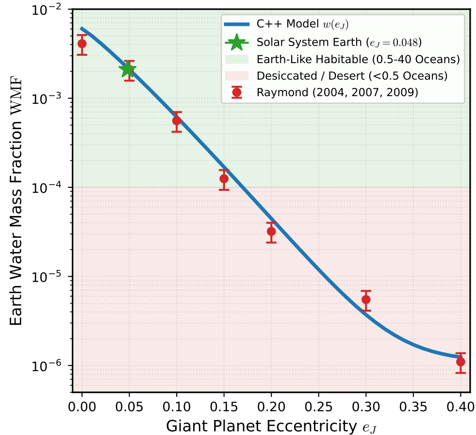
(a) WMF vs. Jupiter Eccentricity ( R^2 = 0.991 )
