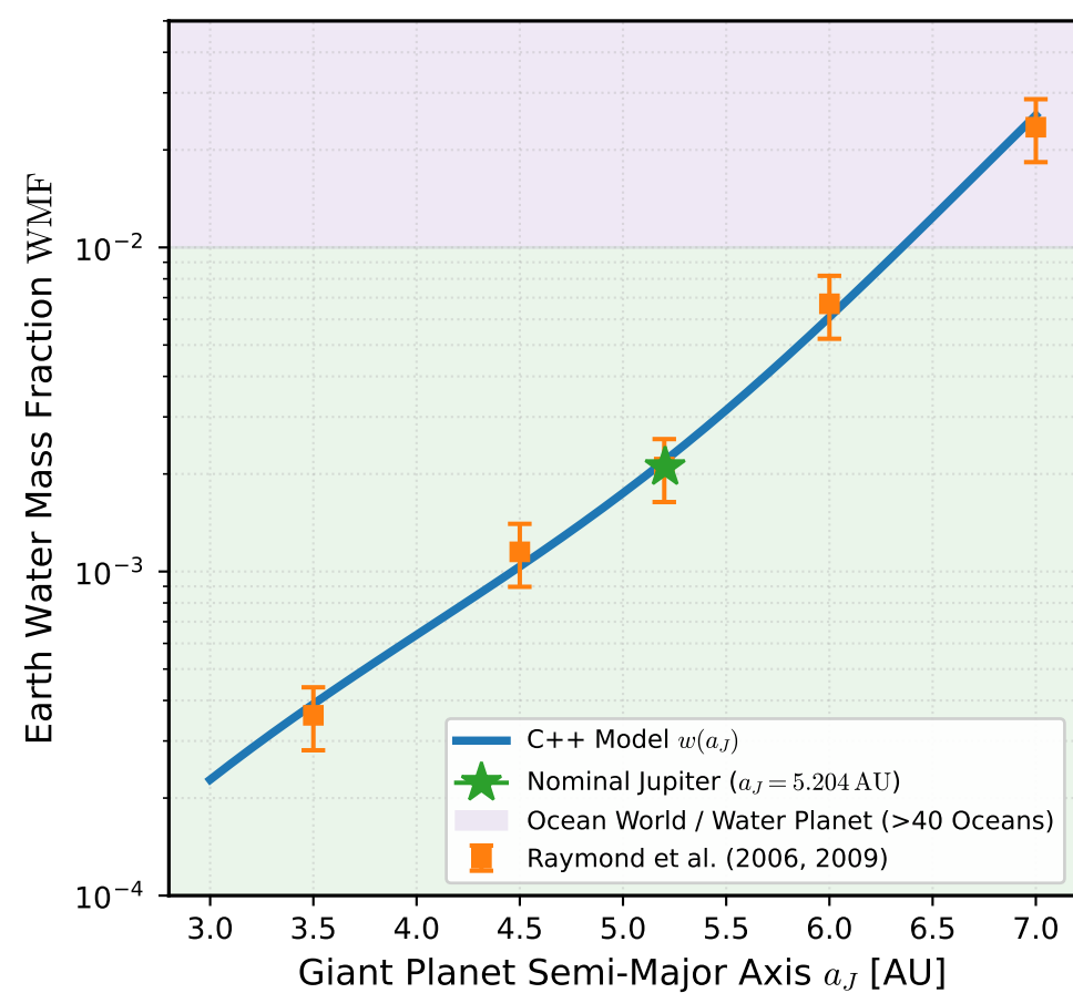
(b) WMF vs. Jupiter Semi-Major Axis ( R^2 = 0.997 )
