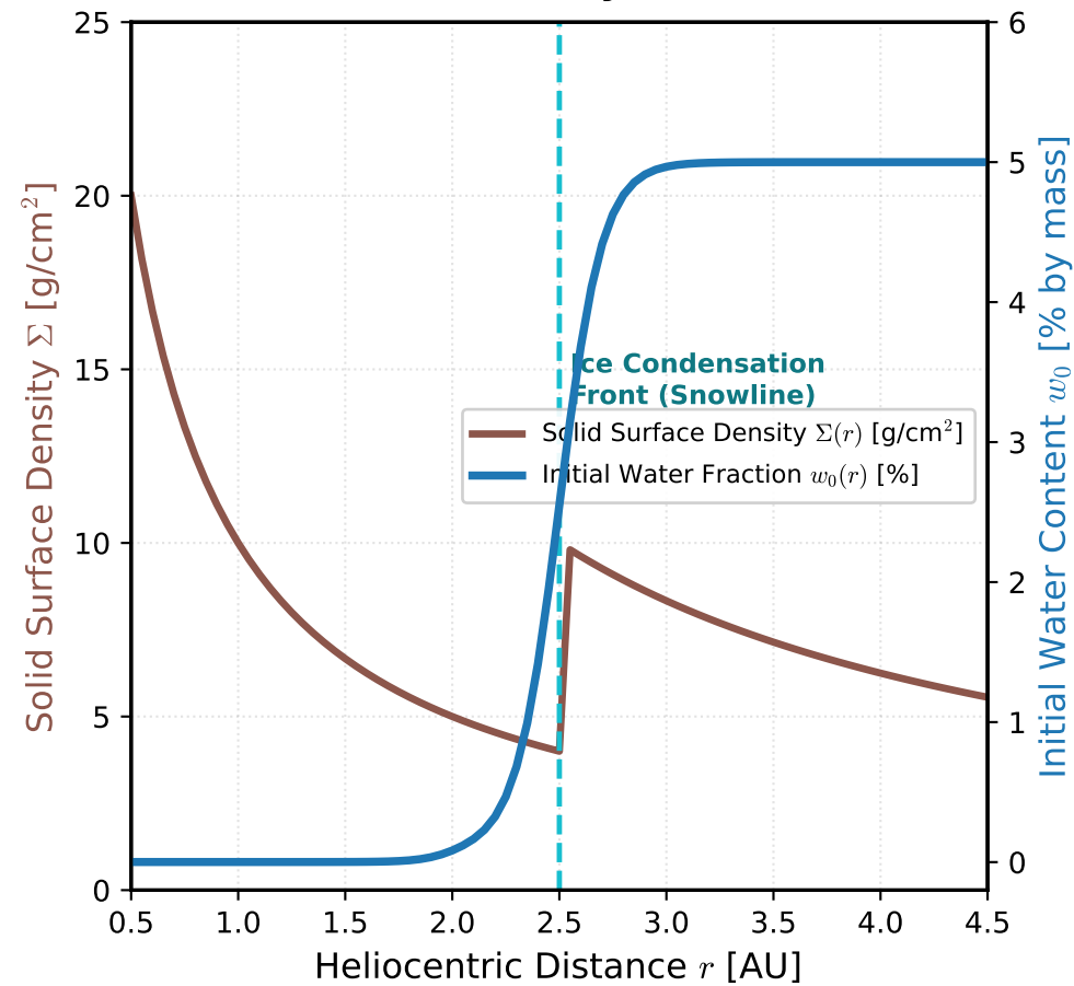
(a) Disk Surface Density & Water Gradient
