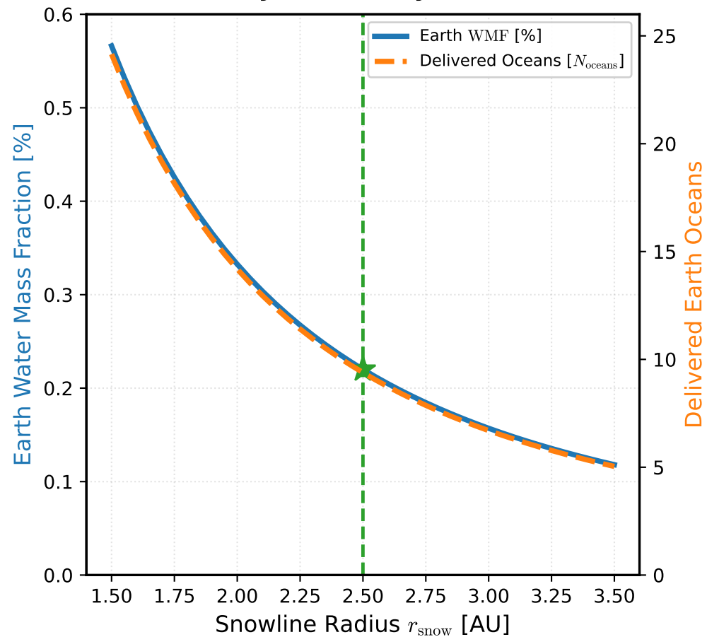
(c) Water Delivery Sensitivity to Snowline Radius
