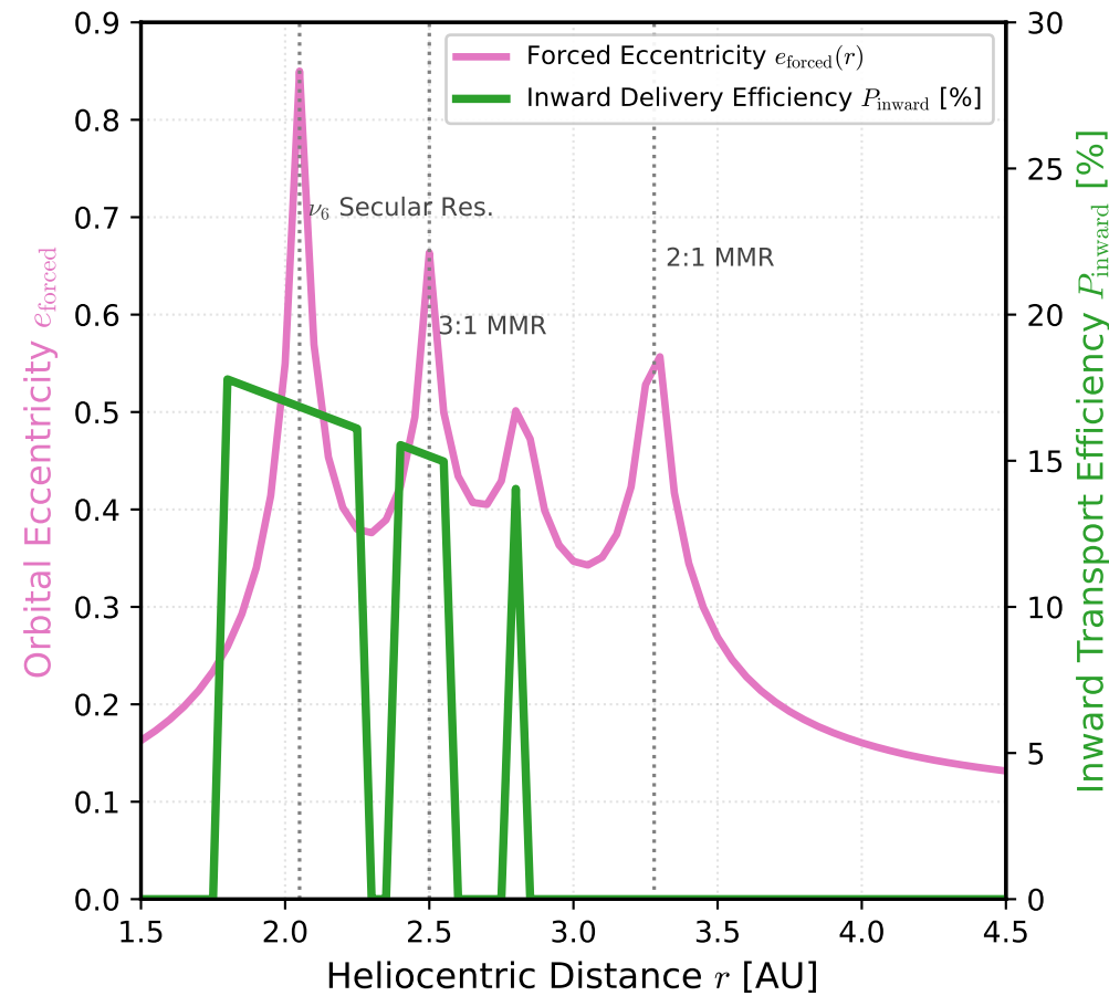
(b) Resonance Excitation & Planetesimal Scattering
