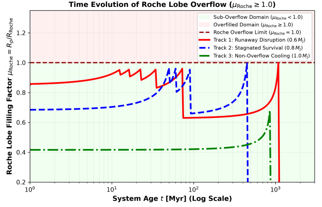
Figure 2: Roche Lobe Radius Contraction and Filling Factor. Time evolution of filling factor \mu_{\text{Roche}}(t) = R_p/R_{\text{Roche}} . Overfilling ( \mu_{\text{Roche}} \geq 1.0 , red shaded region) initiates hydrodynamic mass loss, while sub-overflow ( \mu_{\text{Roche}} < 1.0 , green shaded region) represents stable cooling.
