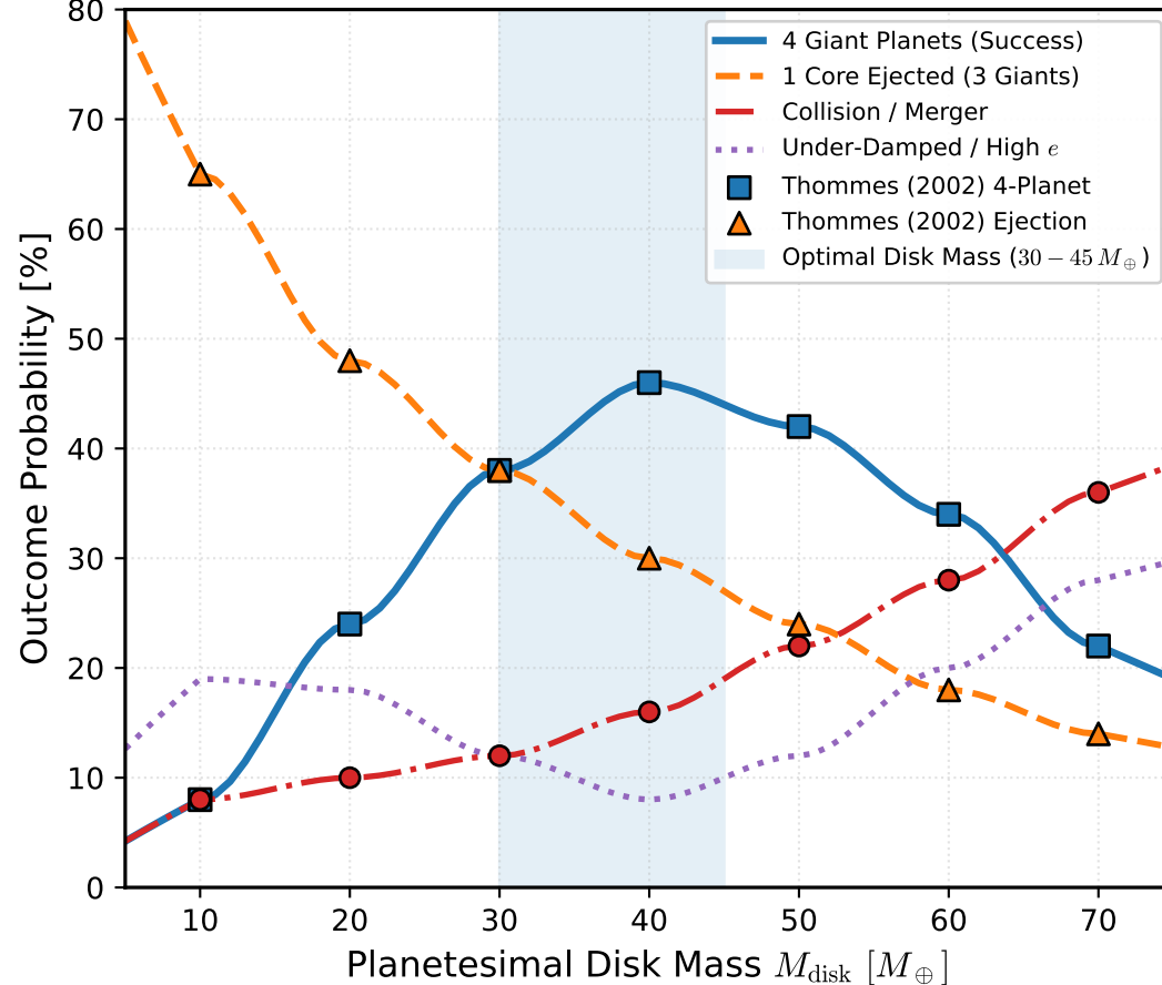
(b) System Architecture Fates vs M_{\text{disk}}
