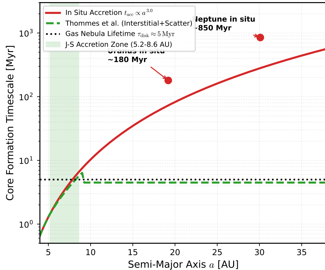
(a) In Situ Core Accretion Crisis vs Distance
