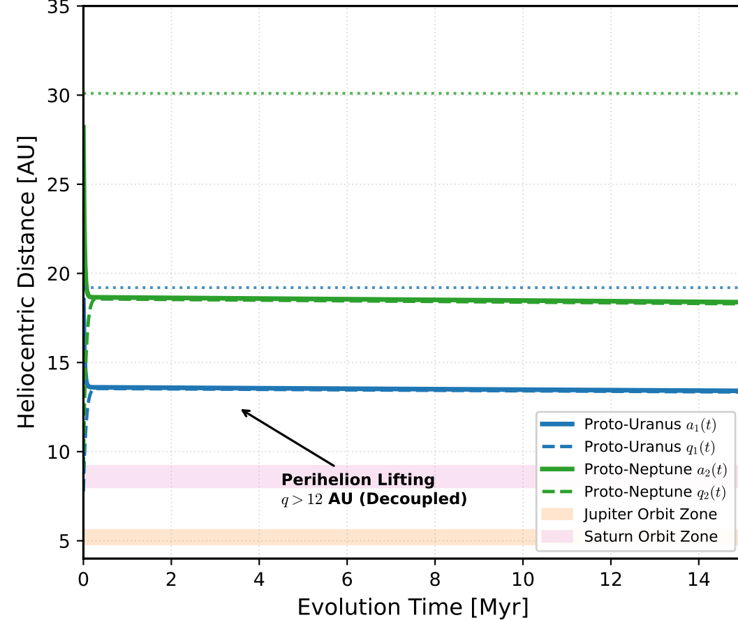
(c) Dynamical Friction & Perihelion Decoupling
