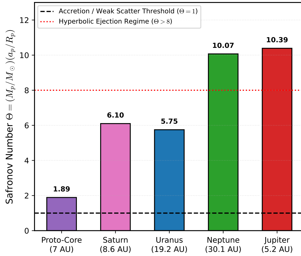
(b) Gravitational Scattering Regimes
