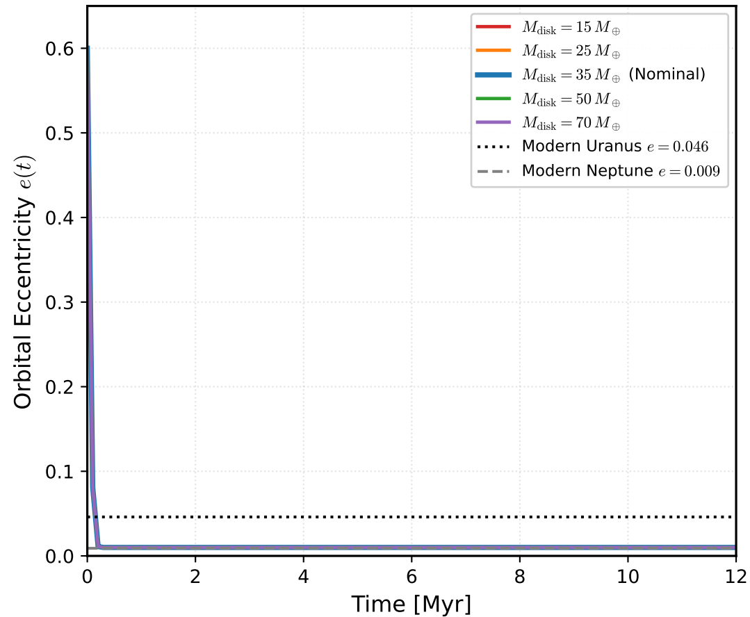
(a) Eccentricity Damping vs Disk Mass M_{\text{disk}}
