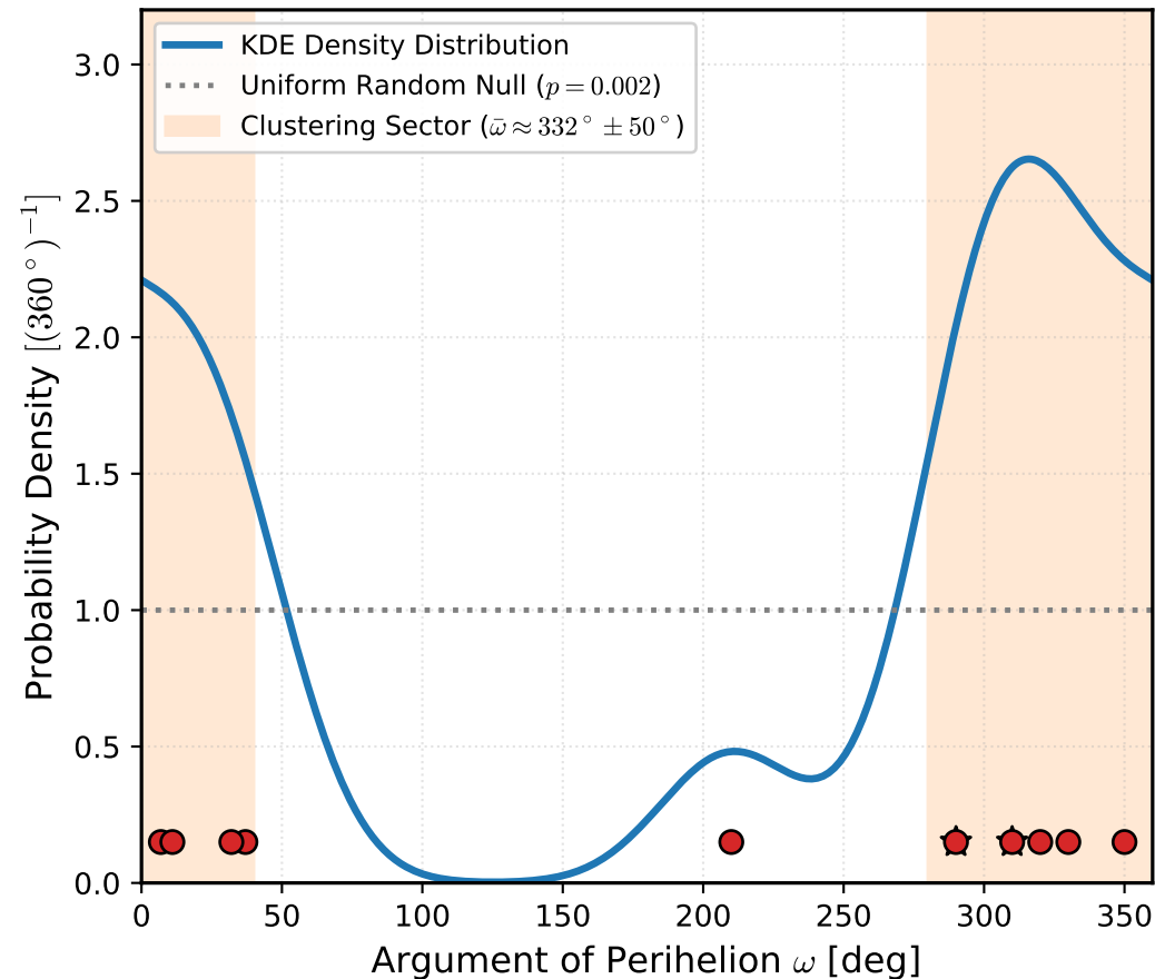
(b) eTNO \omega Clustering ( \bar{\omega} \approx 332^\circ, p = 0.002 )
