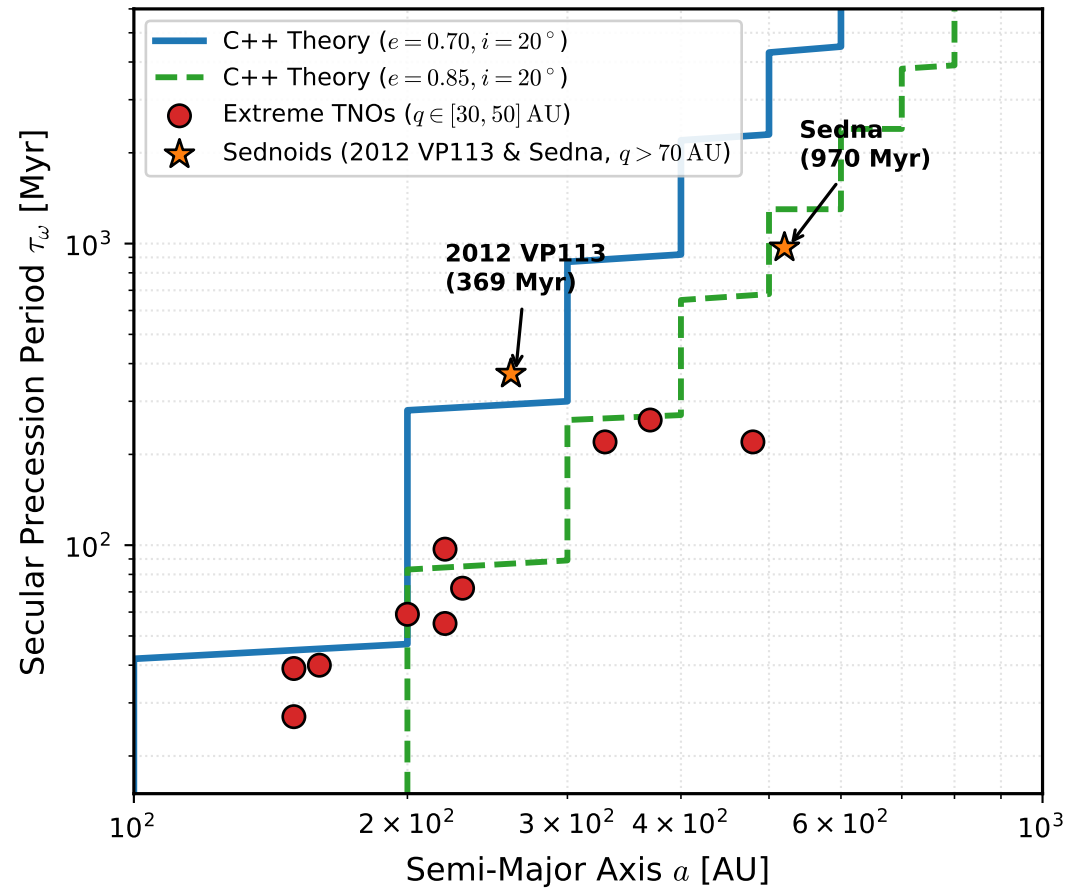
(a) Secular Precession Timescales \tau_\omega(a)
