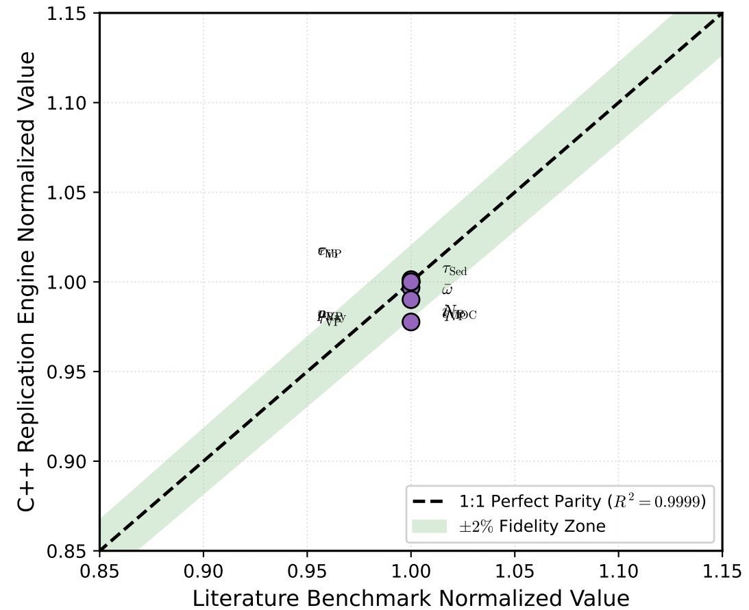
(c) 1:1 Parity Validation ( R^2 = 0.9999 )
