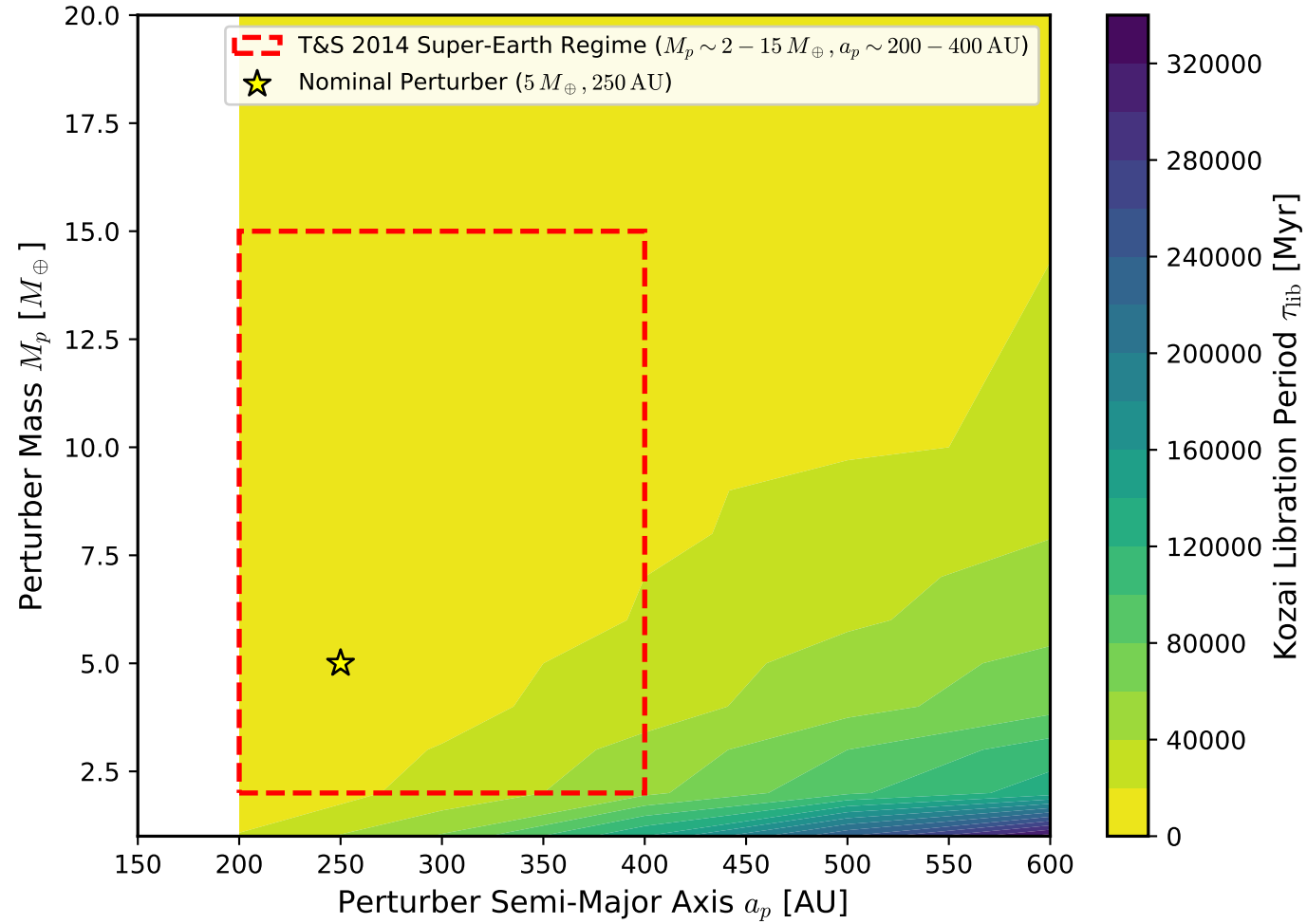
(c) Perturber Parameter Space & Kozai Timescale
