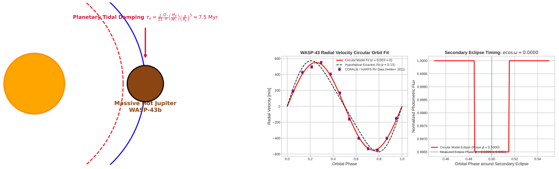
Physical Configuration Diagram: WASP-43b Tidal Eccentricity Circularization
