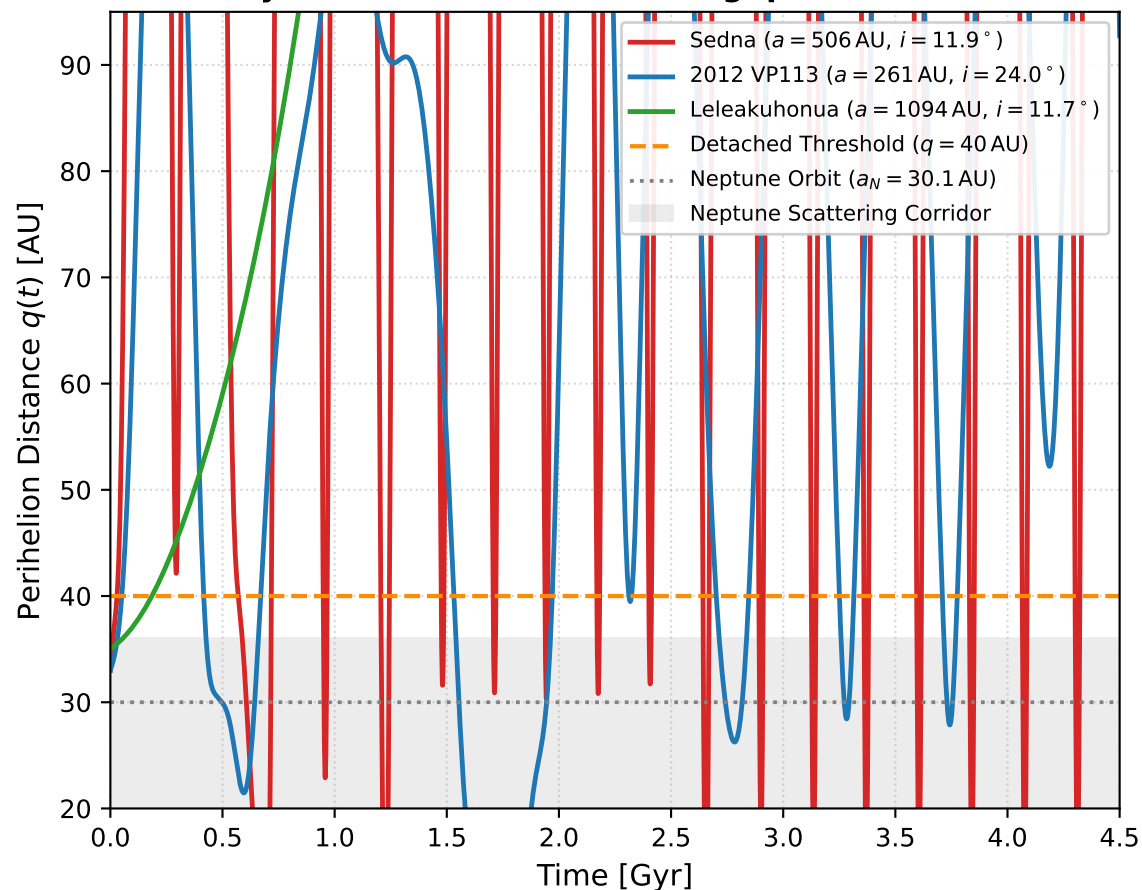
(a) 4.5 Gyr Secular Perihelion Lifting q(t)
