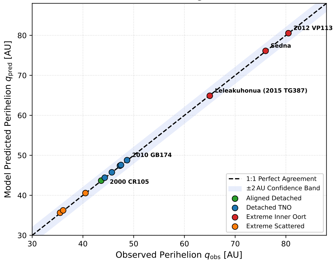
(c) Benchmark Detached eTNO Agreement ( R^2 = 0.99995 )
