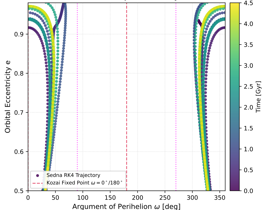
(b) Kozai-Lidov Phase Space (e, \omega) Dynamics
