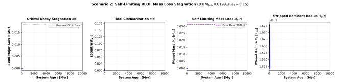
Figure 2: Scenario 2: Self-Limiting RLOF Stagnation ( 0.8 M_{\text{Jup}}, 0.019 \text{ AU}, e_0 = 0.15 ). Coupled time evolution of semi-major axis a(t) , eccentricity e(t) , mass M_p(t) , and radius R_p(t) . Tidal circularization damps eccentricity to zero ( e \rightarrow 0 ), while envelope stripping drives structural contraction ( R_p \propto M_p^{0.6} ), halting mass loss and allowing the planet to survive as a circularized USP remnant.
