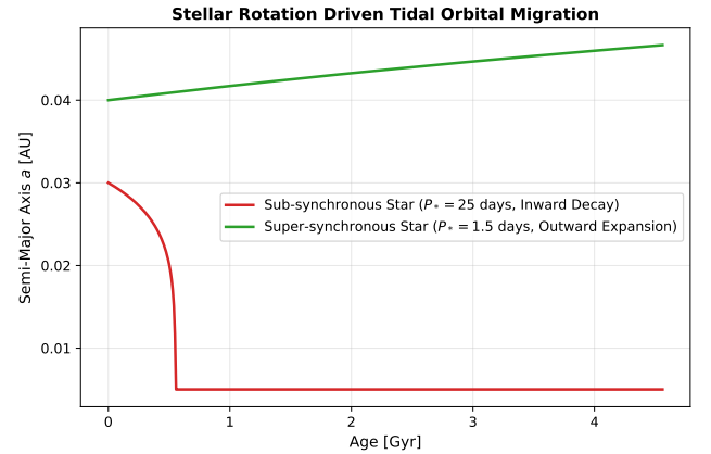
Figure 7: Scenario 6: Sub-synchronous inward orbital decay vs super-synchronous outward orbital expansion driven by host star rotation.
