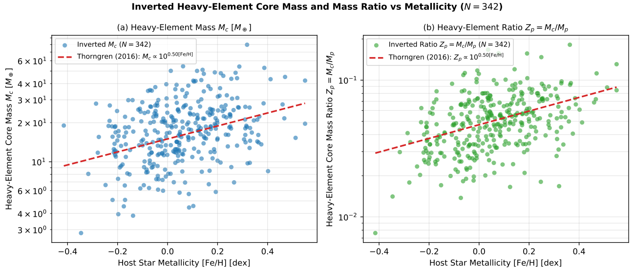
Figure 13: Dual-panel core mass inversion analysis across all N = 342 confirmed transiting Hot Jupiters: (a) Absolute heavy-element core mass M_c [ M_\oplus ] vs host star metallicity [Fe/H] [dex], and (b) Dimensionless heavy-element core mass fraction Z_p = M_c/M_p vs [Fe/H] [dex], compared against the empirical Thorngren et al. (2016) power-law trend.
