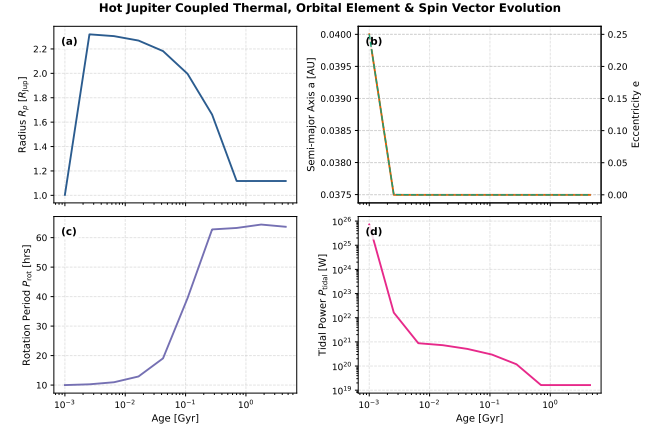
Figure 3: Scenario 2: Coupled thermal, orbital element ( a, e ), and 3D spin vector ( \Omega_{\text{rot}}, \varepsilon ) evolution for a Hot Jupiter over 4.56 \text{ Gyr} , illustrating tidal circularization, spin synchronization, and radius inflation retardation.
