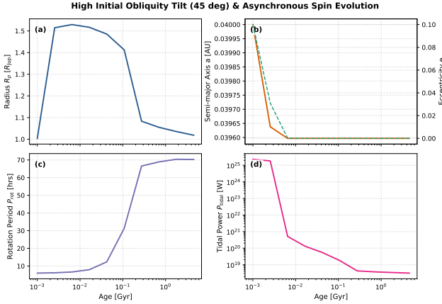
Figure 5: Scenario 4: High initial obliquity tilt ( 45^\circ ) and asynchronous rotation trajectory over 4.56 Gyr.
