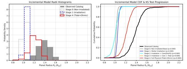
Figure 9: Scenario 8: Cumulative Distribution Function (CDF) and Kolmogorov-Smirnov (KS) metric comparison between baseline cooling models, interior heating models, and empirical exoplanet observations.
