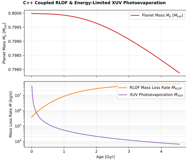
Figure 11: Scenario 10: Coupled planetary mass decay M_p(t) and mass loss rate components ( \dot{M}_{RLOF} vs \dot{M}_{XUV} ) over 4.56 Gyr.
