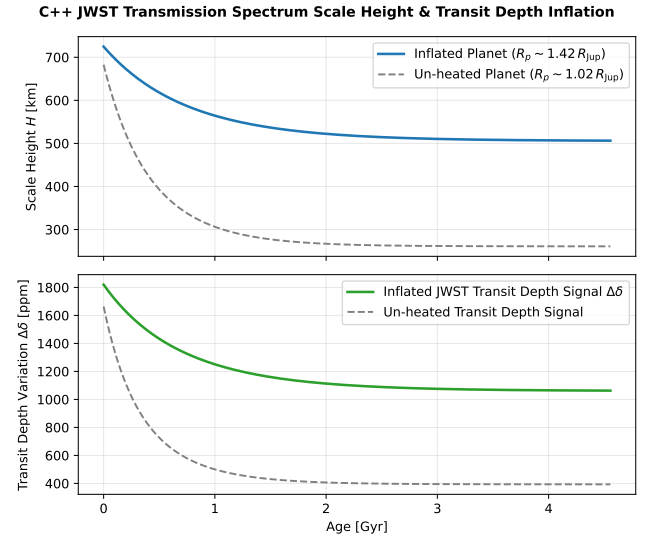
Figure 10: Scenario 9: Atmospheric scale height inflation H(t) and JWST transmission spectrum transit depth signal variations \Delta\delta(t) over 4.56 Gyr.
