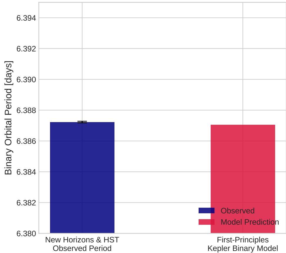
Pluto-Charon Orbital Period Comparison
