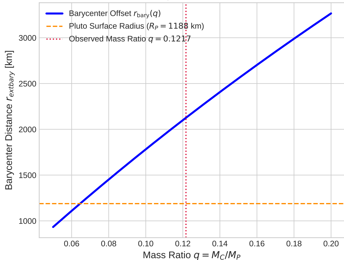
Model Choice: Barycenter Offset vs Mass Ratio
