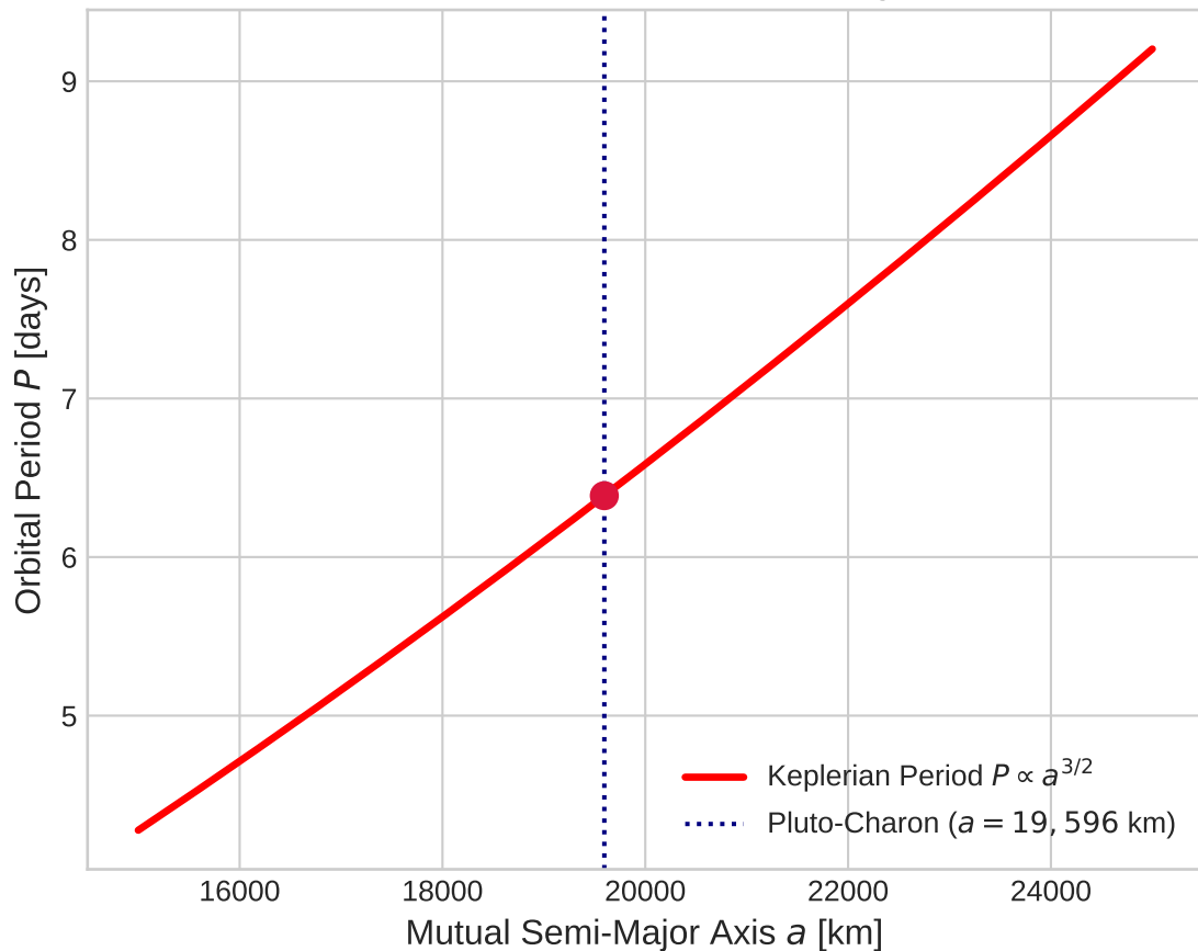
Model Choice: Period vs Semi-Major Axis
