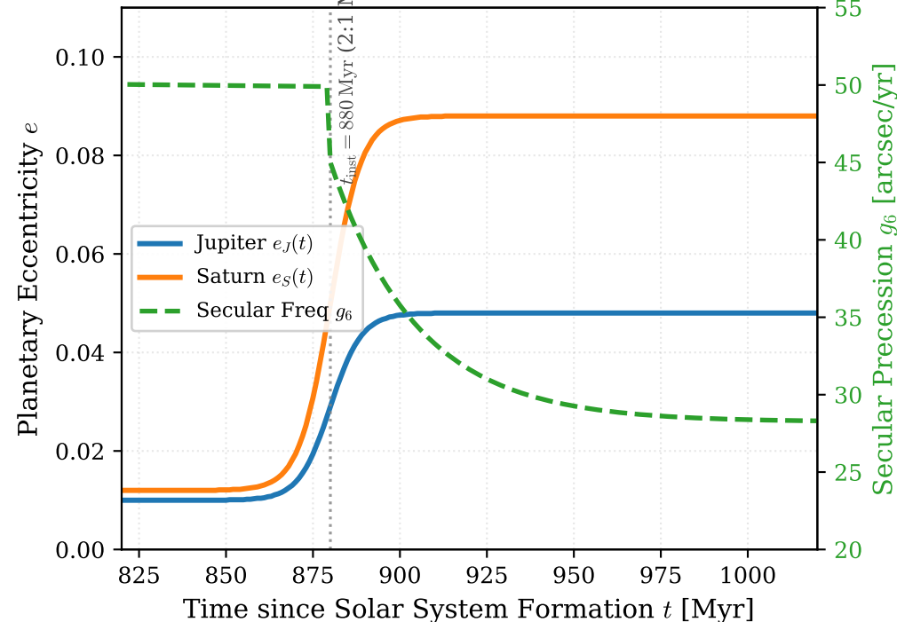
(a) 2:1 Jupiter-Saturn MMR Crossing & Eccentricity Jump
