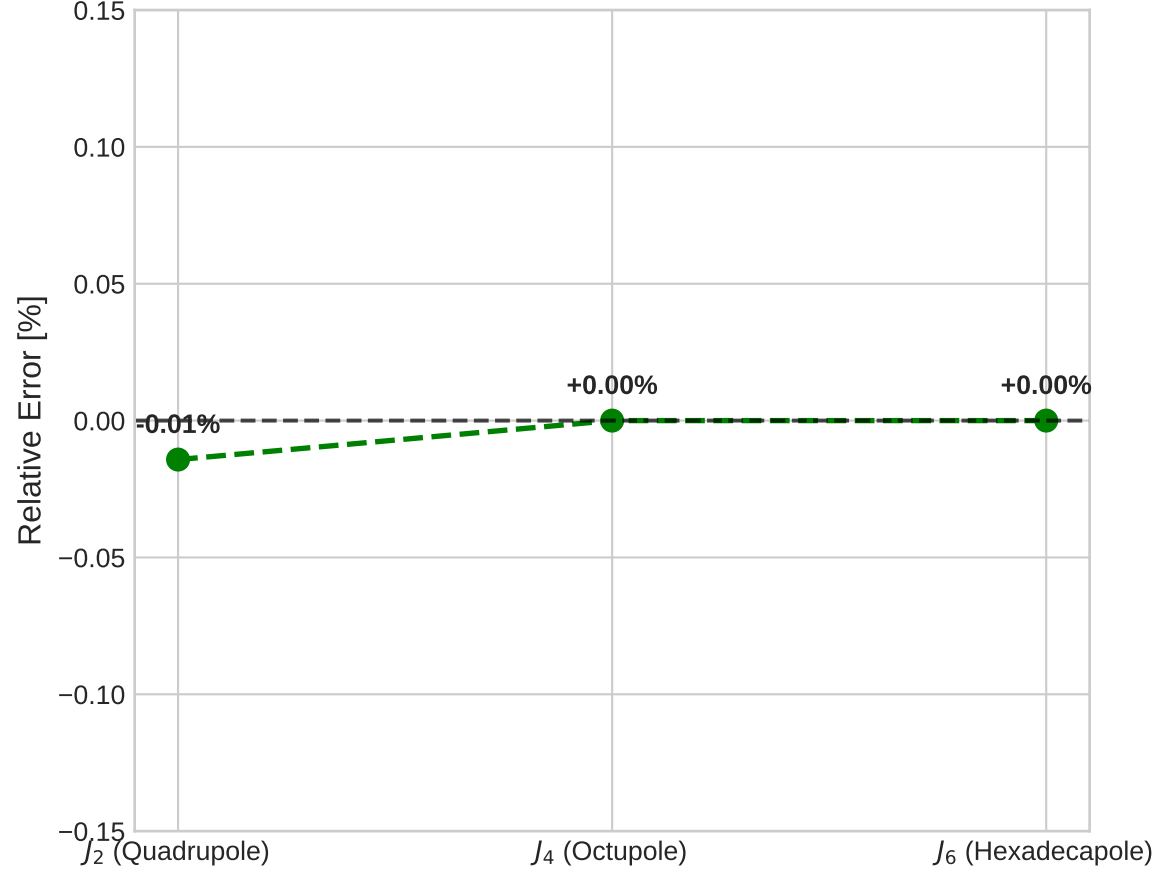
Model Residual Error Relative to Cassini Measurements
