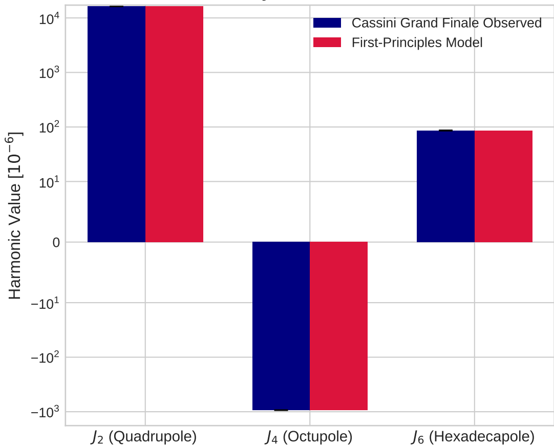
Saturn Zonal Gravity Harmonics: Cassini vs Model
