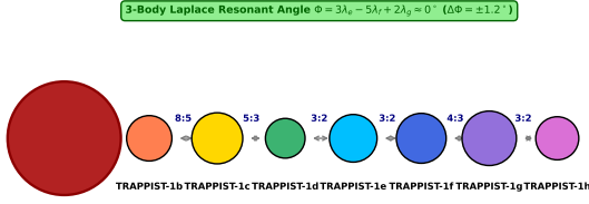
Physical Configuration Diagram: TRAPPIST-1 Seven-Planet Resonant Laplace Chain
