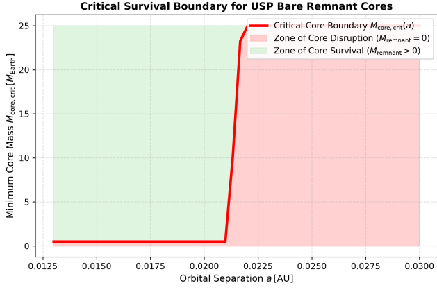
Figure 7: Critical Survival Boundary for USP Remnants. Minimum core mass threshold M_{\text{core, crit}}(a) separating complete core disruption (red shaded region) from stable core survival (green shaded region).
