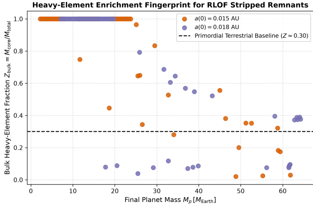
Figure 8: Heavy-Element Enrichment Fingerprint. Final bulk heavy-element fraction Z_{\text{bulk}} \equiv M_{\text{core}}/M_{\text{total}} of surviving USP remnants, compared against the baseline of primordially accreted terrestrial planets ( Z \approx 0.30 ).
