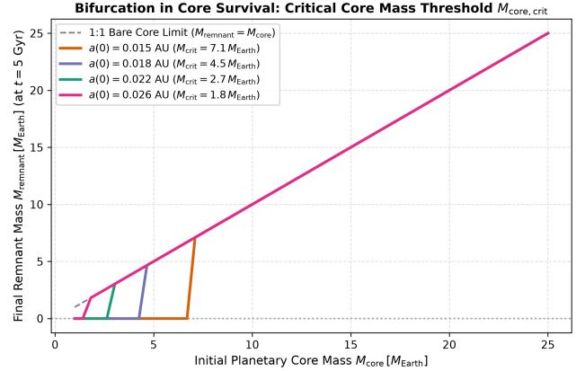
Figure 6: Bifurcation in Core Survival. Final remnant mass M_{remnant} at t = 5 Gyr as a function of initial core mass M_{core} across orbital separations a(0) \in [0.015, 0.026] AU. Cores below M_{core, crit} undergo total hydrodynamic disruption ( M_{remnant} = 0 ).
