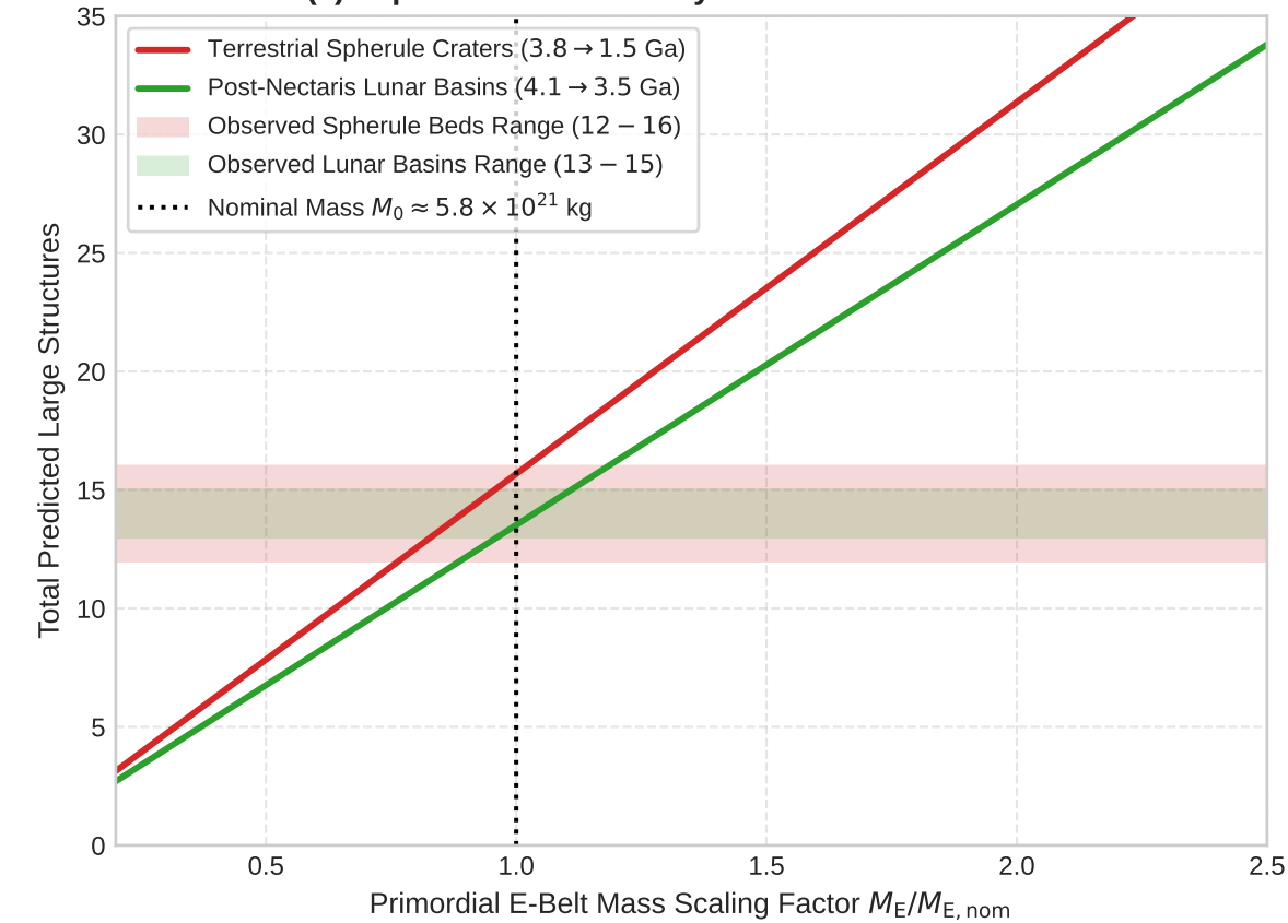
(c) Impact Yield Sensitivity to Primordial Belt Mass
