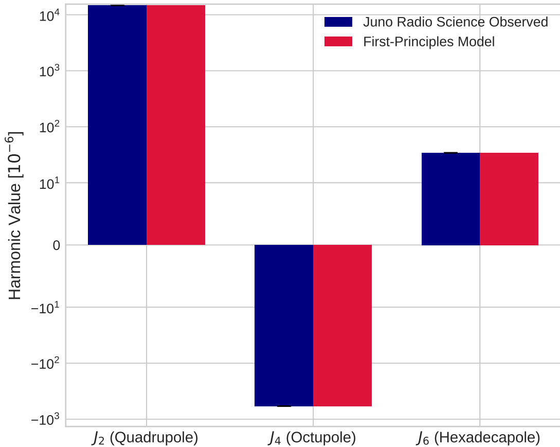
Jupiter Zonal Gravity Harmonics: Juno vs Model
