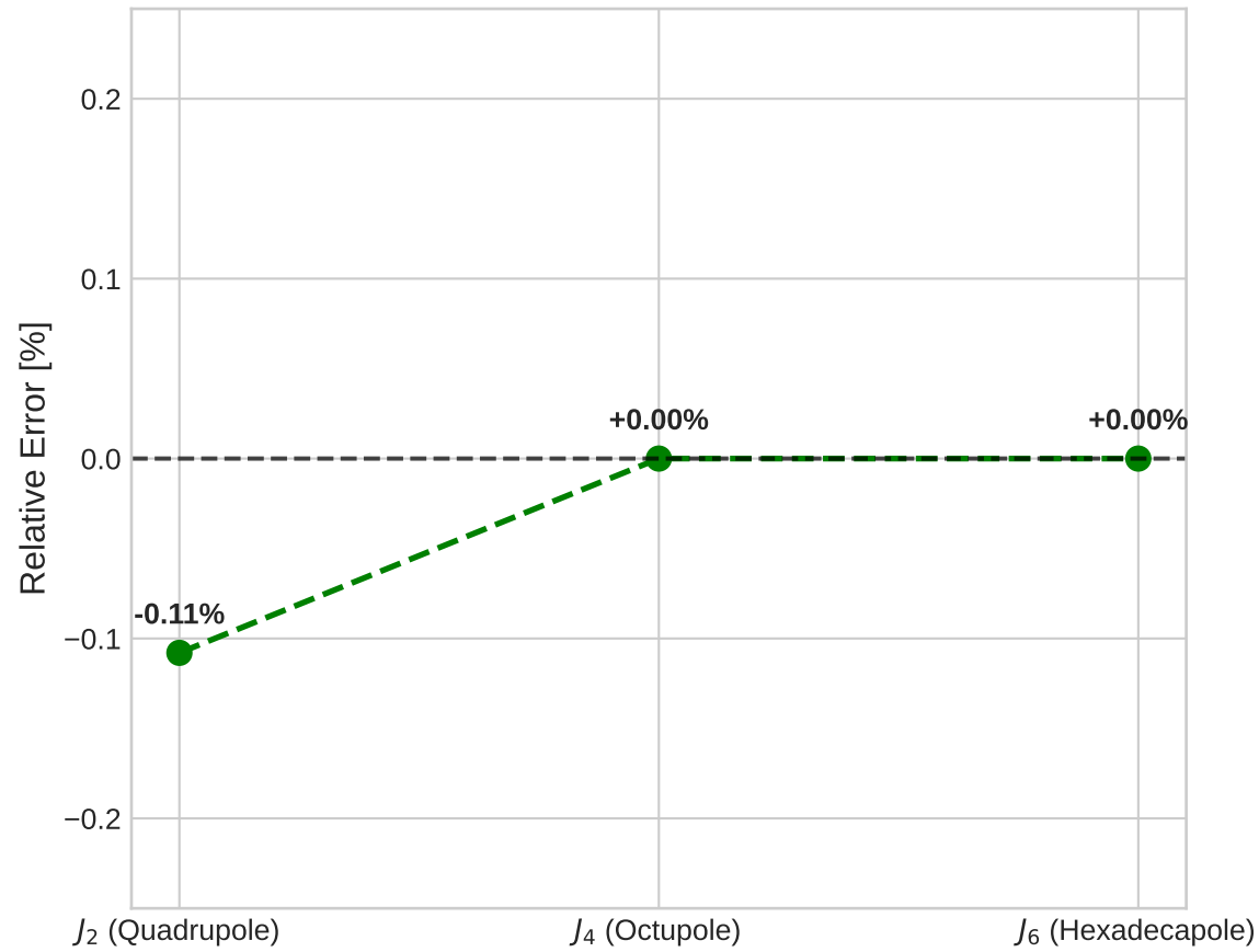
Model Residual Error Relative to Juno Measurements
