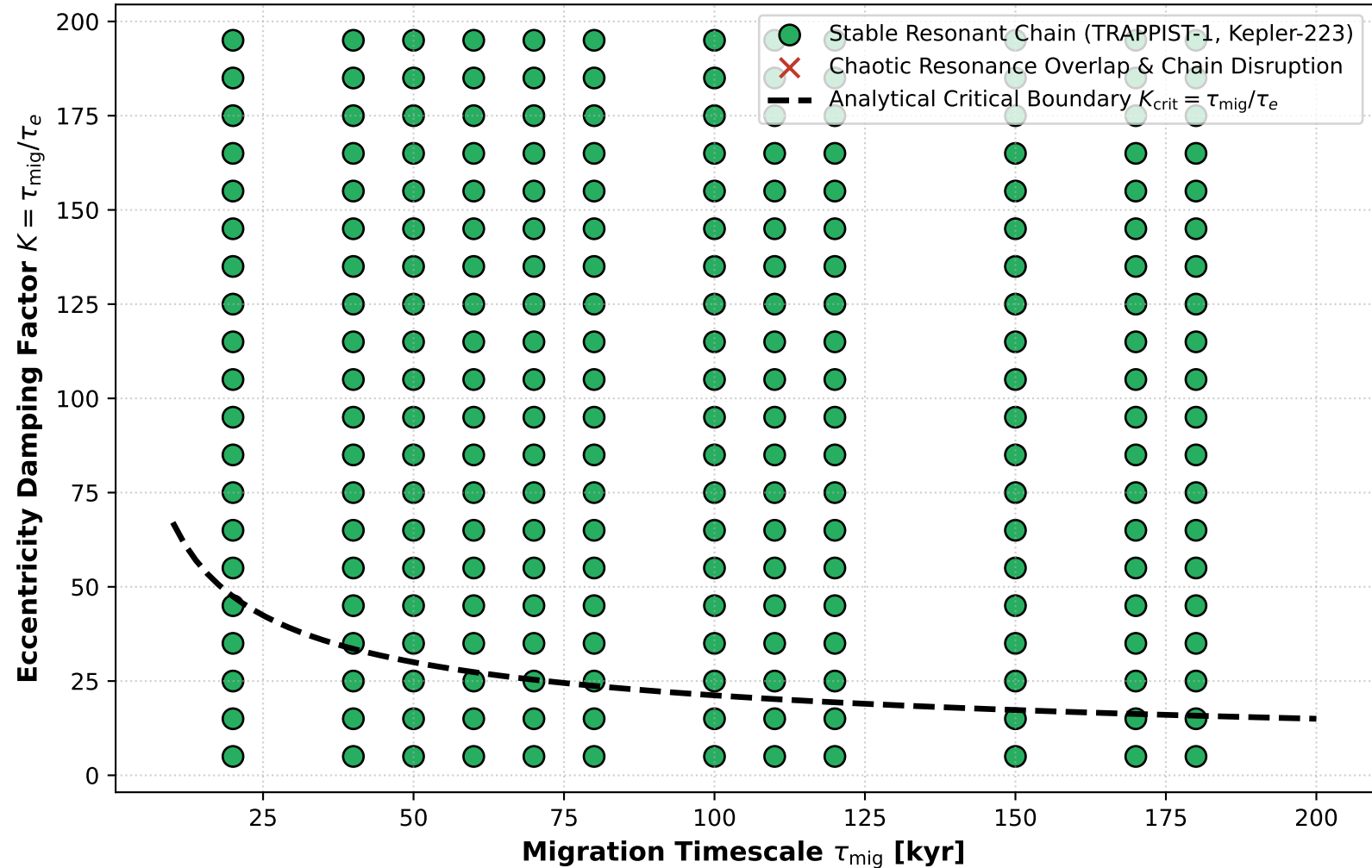
Frontier 5 Phase Diagram: Resonant Chain Survival vs. Chaotic Dissolution
