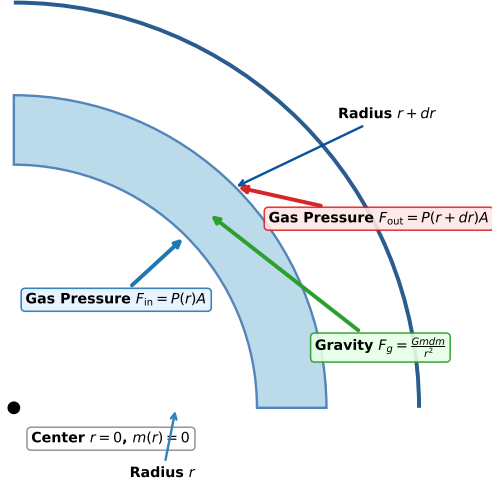
Figure 14: 1D Hydrostatic shell force balance between gas pressure gradients and self-gravity.
