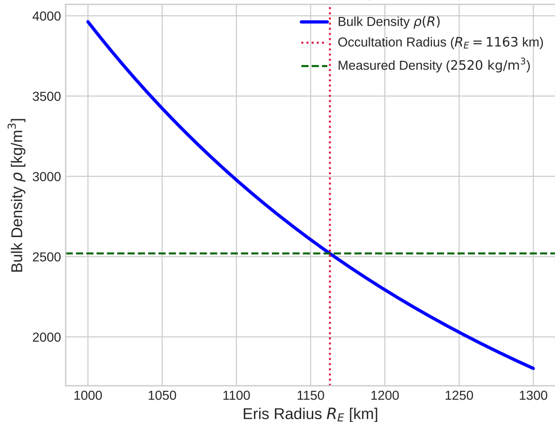
Model Choice: Bulk Density Sensitivity
