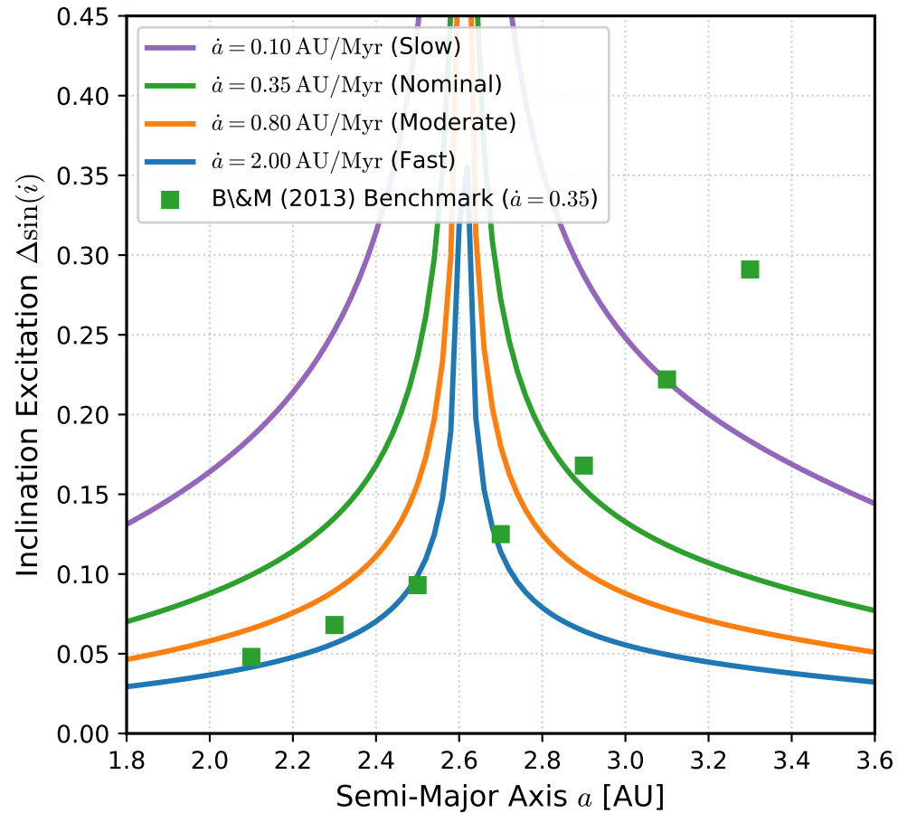
(b) Analytical Inclination Kick \Delta \sin(i)
