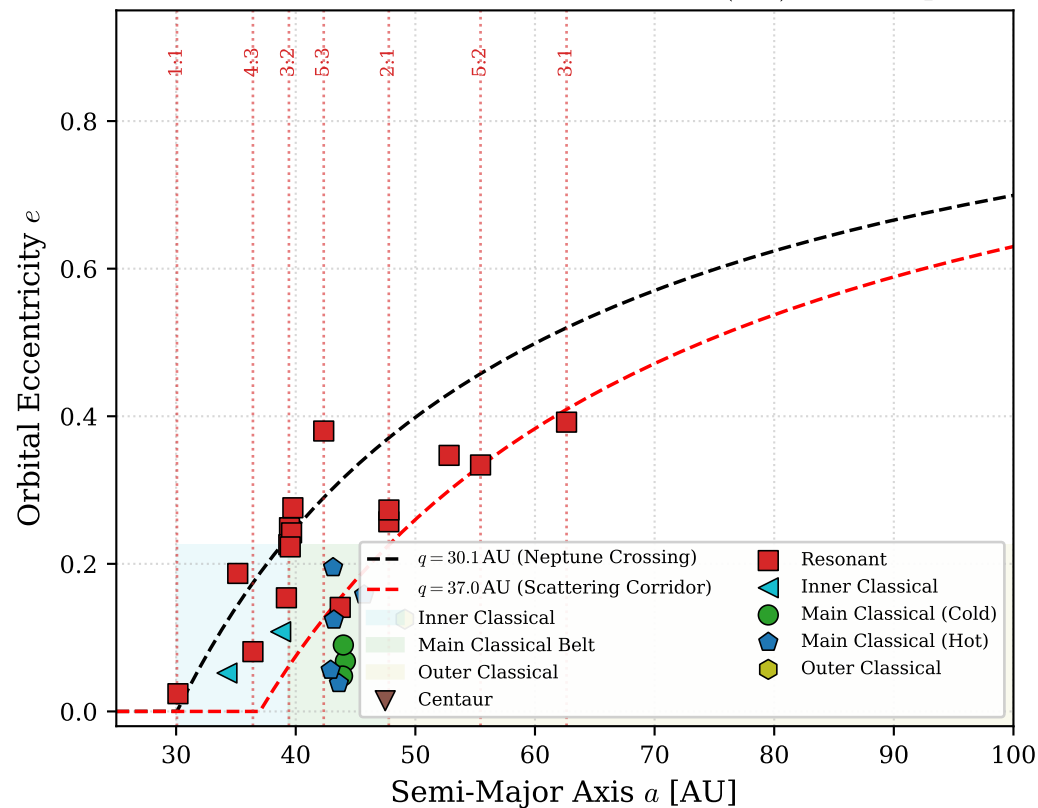
(a) TNO Orbital Distribution in (a, e) Phase Space
