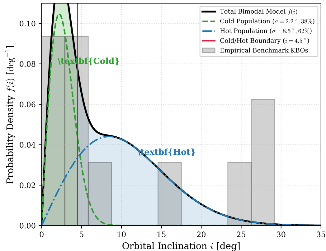
(b) Classical Belt Bimodal Inclination Distribution f(i)
