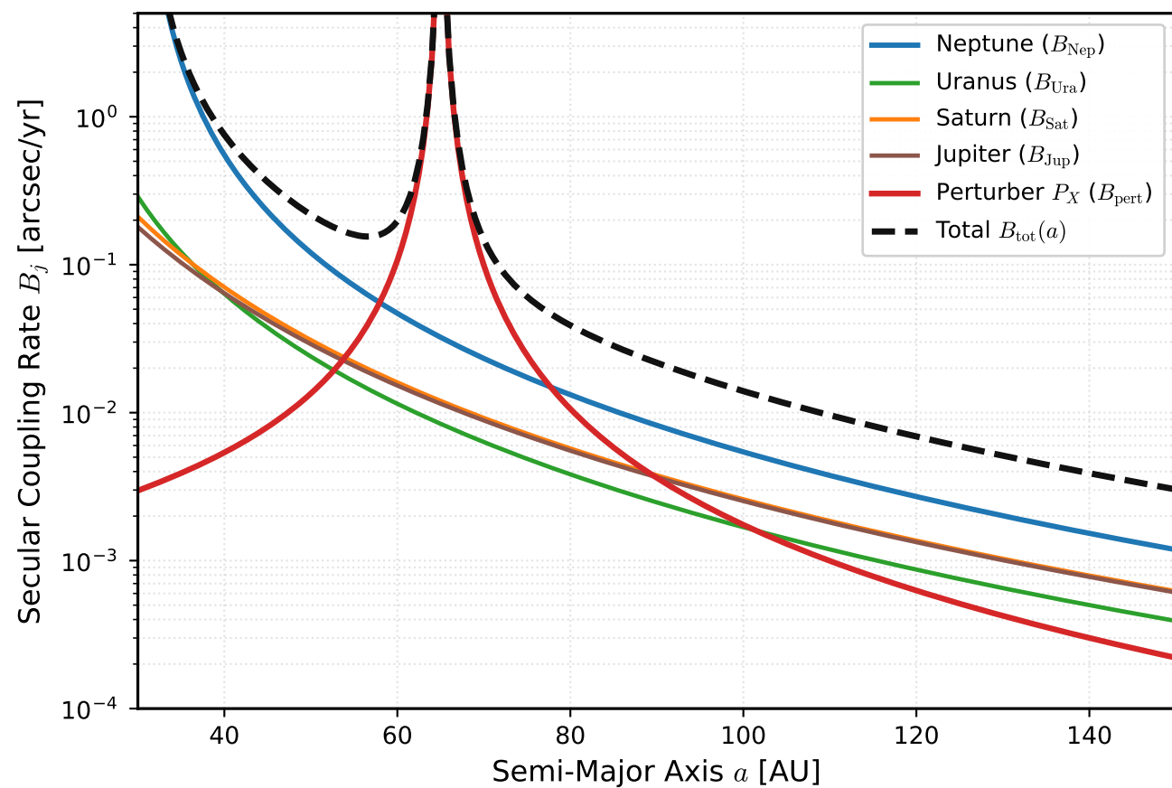
(c) Secular Precession Frequency Breakdown
