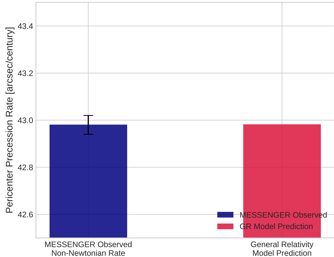
Non-Newtonian Pericenter Advance Comparison
