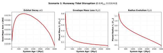
Figure 1: Scenario 1: Runaway Tidal Disruption ( 0.6 M_{\text{Jup}} , 0.016 \text{ AU} ). Coupled time evolution of orbital semi-major axis a(t) , planetary mass M_p(t) , and radius R_p(t) during runaway envelope mass loss and tidal engulfment into the star.
