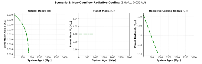
Figure 3: Scenario 3: Non-Overflow Radiative Cooling ( 1.0 M_{\text{Jup}} , 0.030 \text{ AU} ). Coupled evolution of semi-major axis a(t) , mass M_p(t) , and radius R_p(t) for a planet that remains sub-overflow ( \mu_{\text{Roche}} < 1 ), retaining its primordial envelope while undergoing standard thermal contraction.
