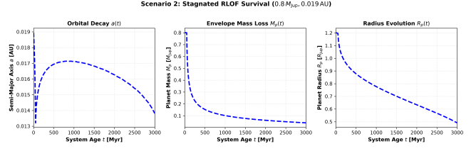
Figure 2: Scenario 2: Self-Limiting RLOF Stagnation ( 0.8 M_{\text{Jup}} , 0.019 \text{ AU} ). Coupled time evolution of semi-major axis a(t) , mass M_p(t) , and radius R_p(t) . Rapid outer envelope stripping drives structural contraction ( R_p \propto M_p^{0.6} ), halting mass loss and enabling planet survival.
