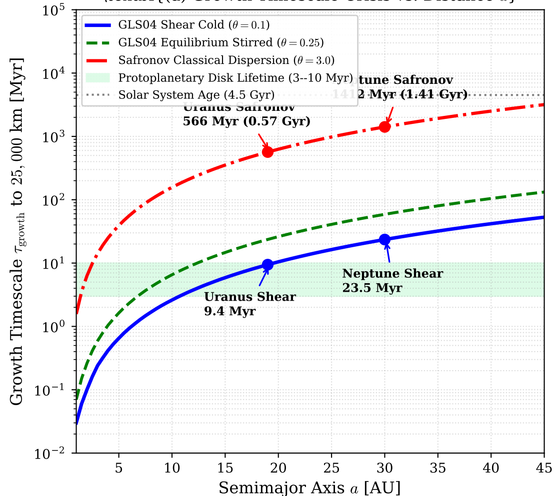
(a) Growth Timescale Crisis vs. Distance a
