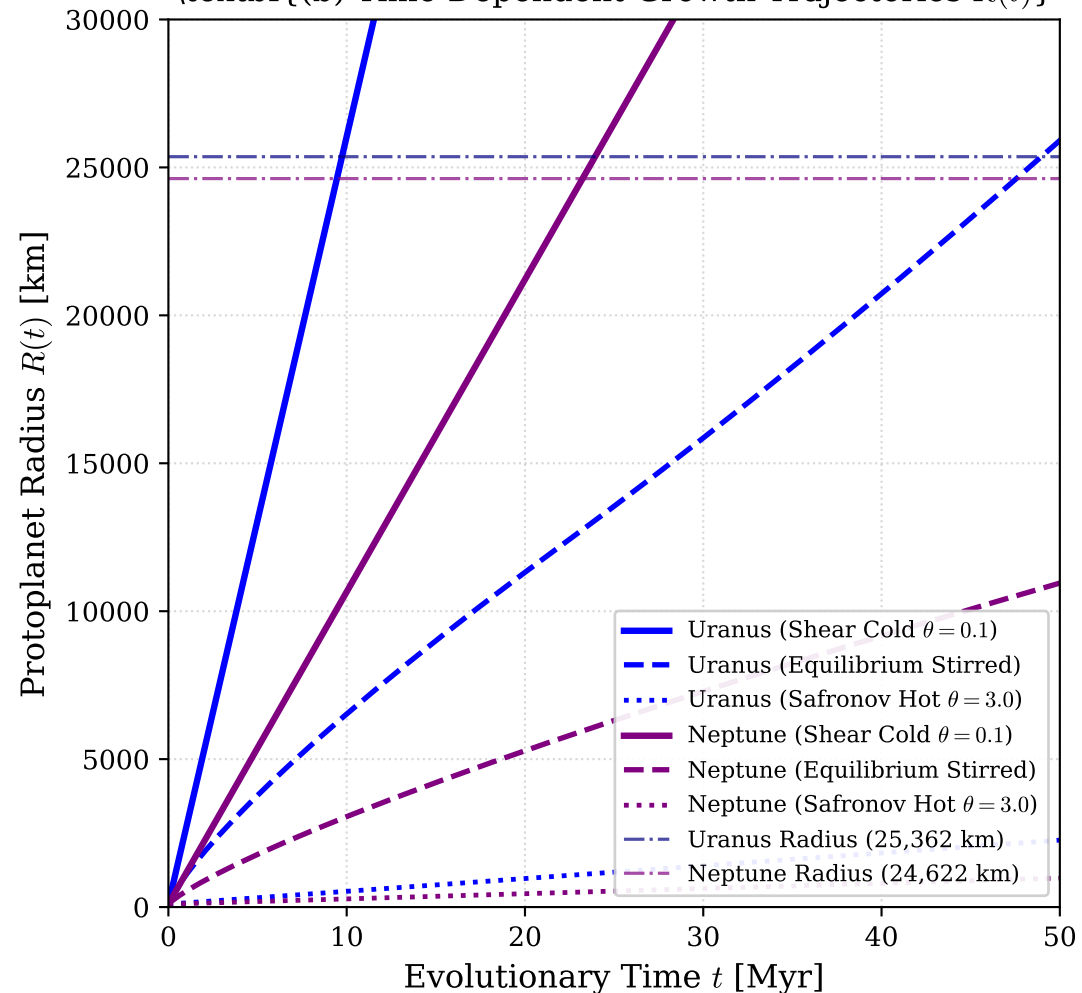
(b) Time-Dependent Growth Trajectories R(t)
