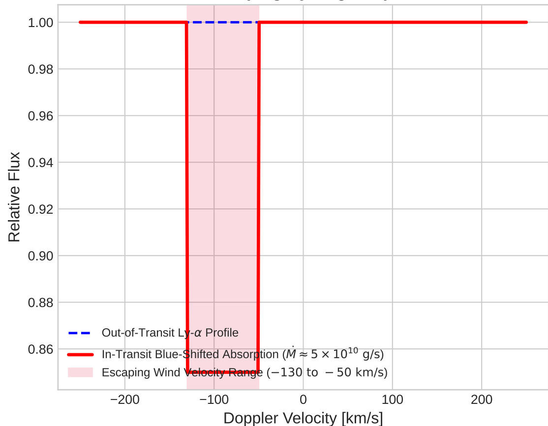
Blue-Shifted Escaping Hydrogen Spectral Feature
