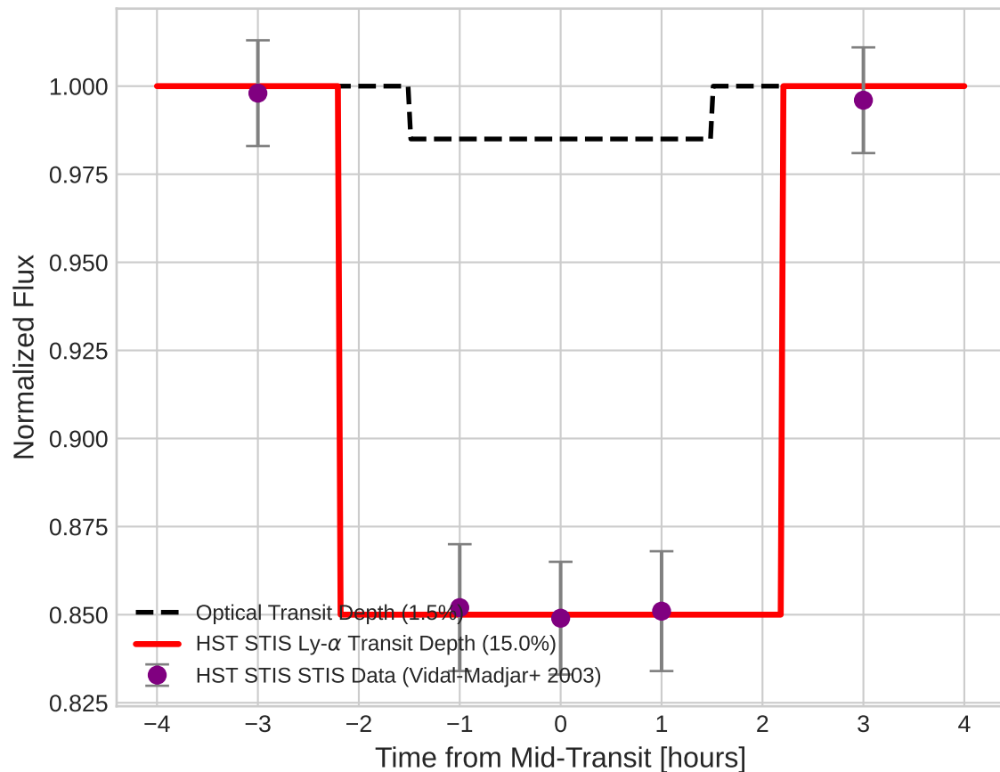
HD 209458b STIS Ly- \alpha Transit Light Curve
