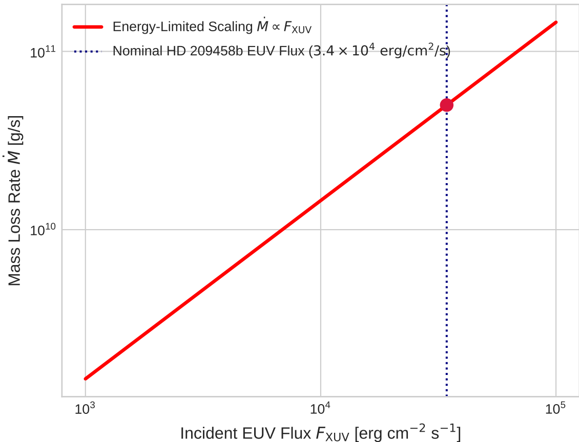
Model Choice: Mass Loss vs Stellar EUV Flux
