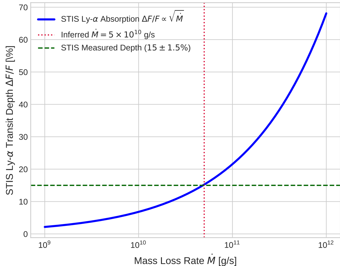
Model Choice: Ly- \alpha Transit Depth Sensitivity
