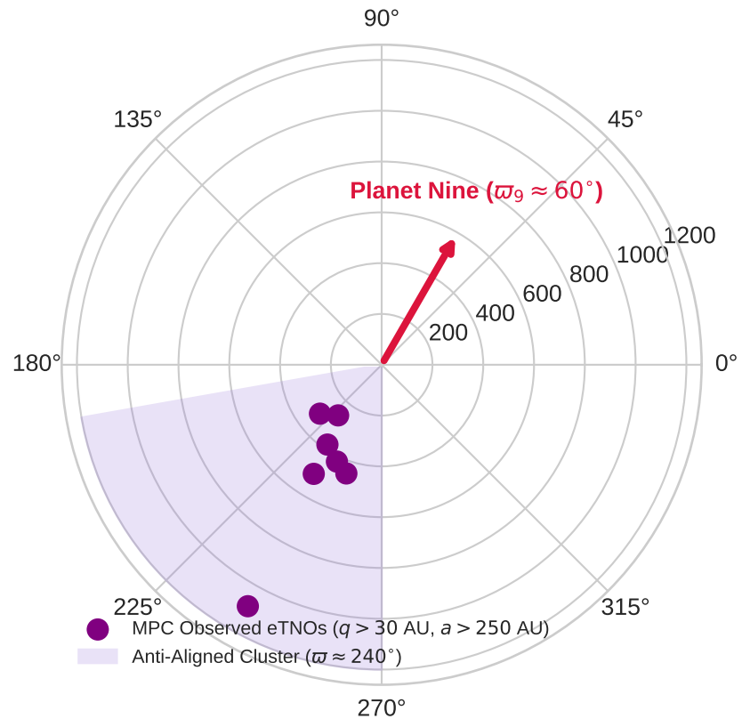
MPC eTNO Longitude of Perihelion ( \varpi ) Alignment
