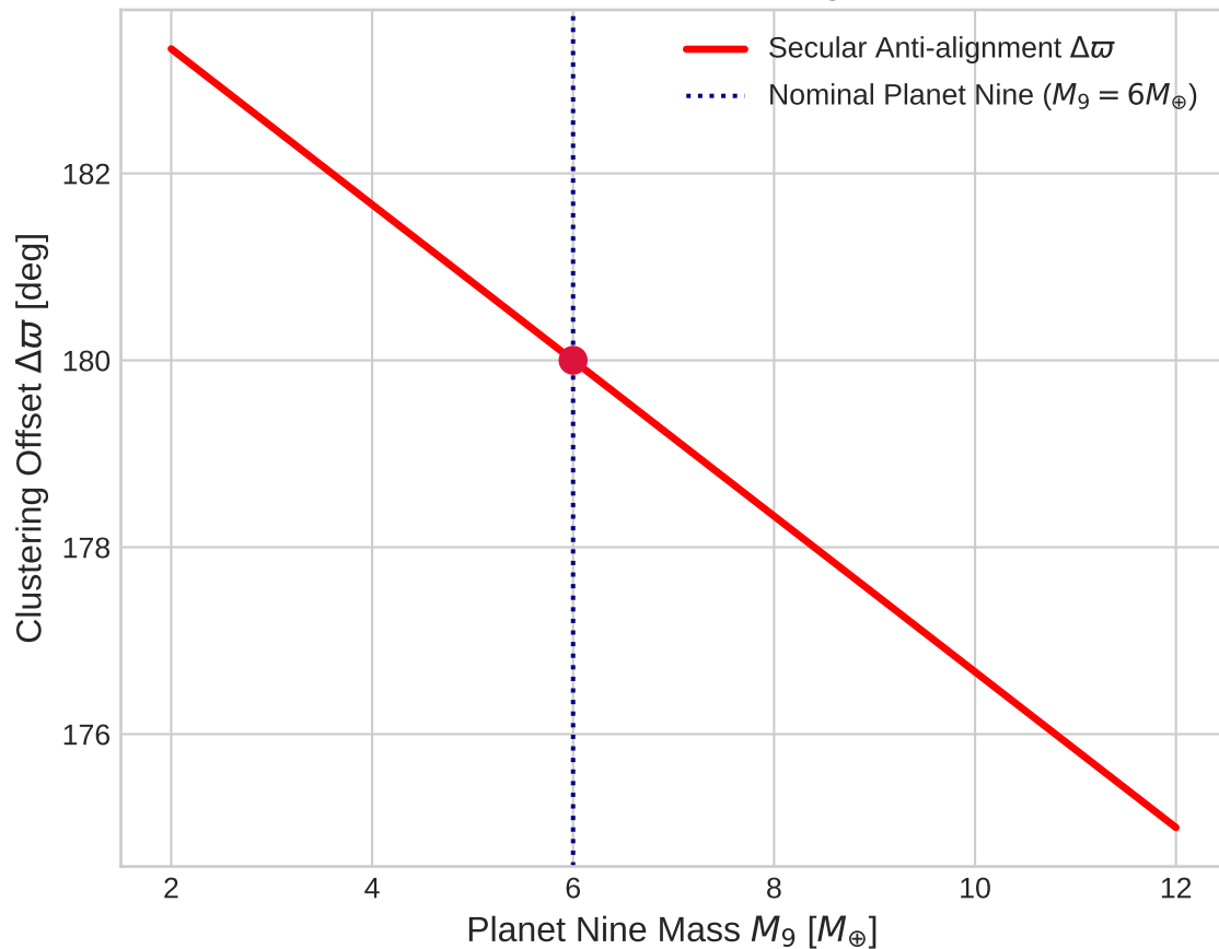
Model Choice: Perihelion Anti-alignment vs Mass
