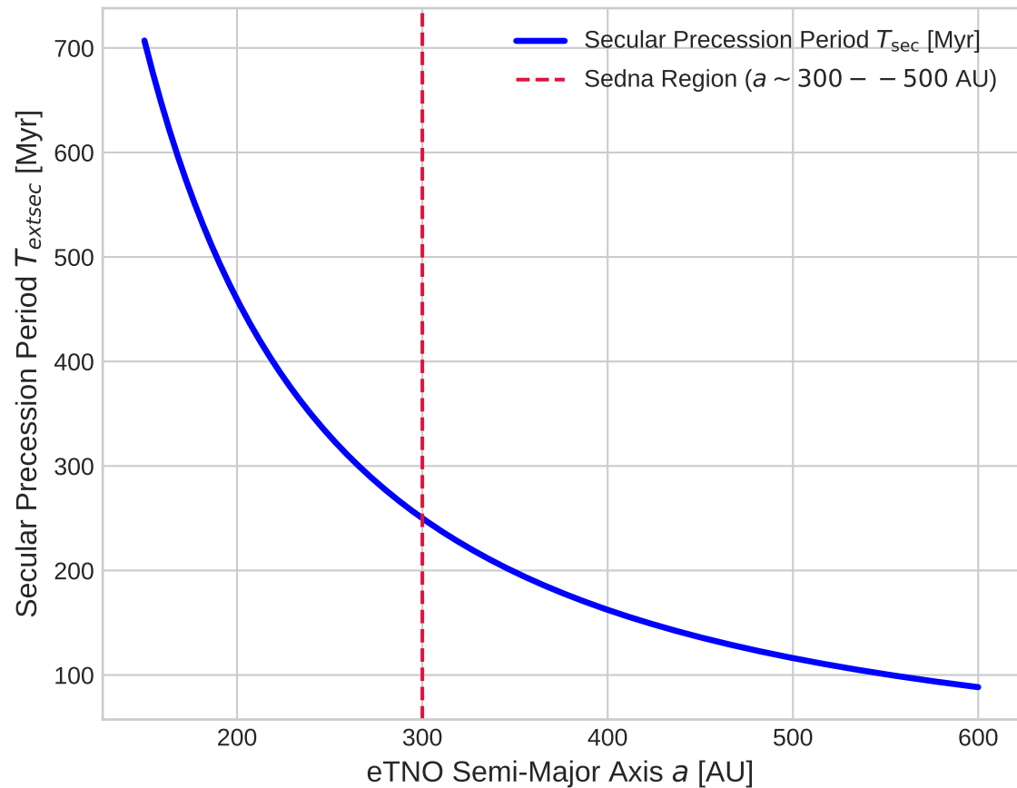
Secular Precession Timescale vs Orbit Size
