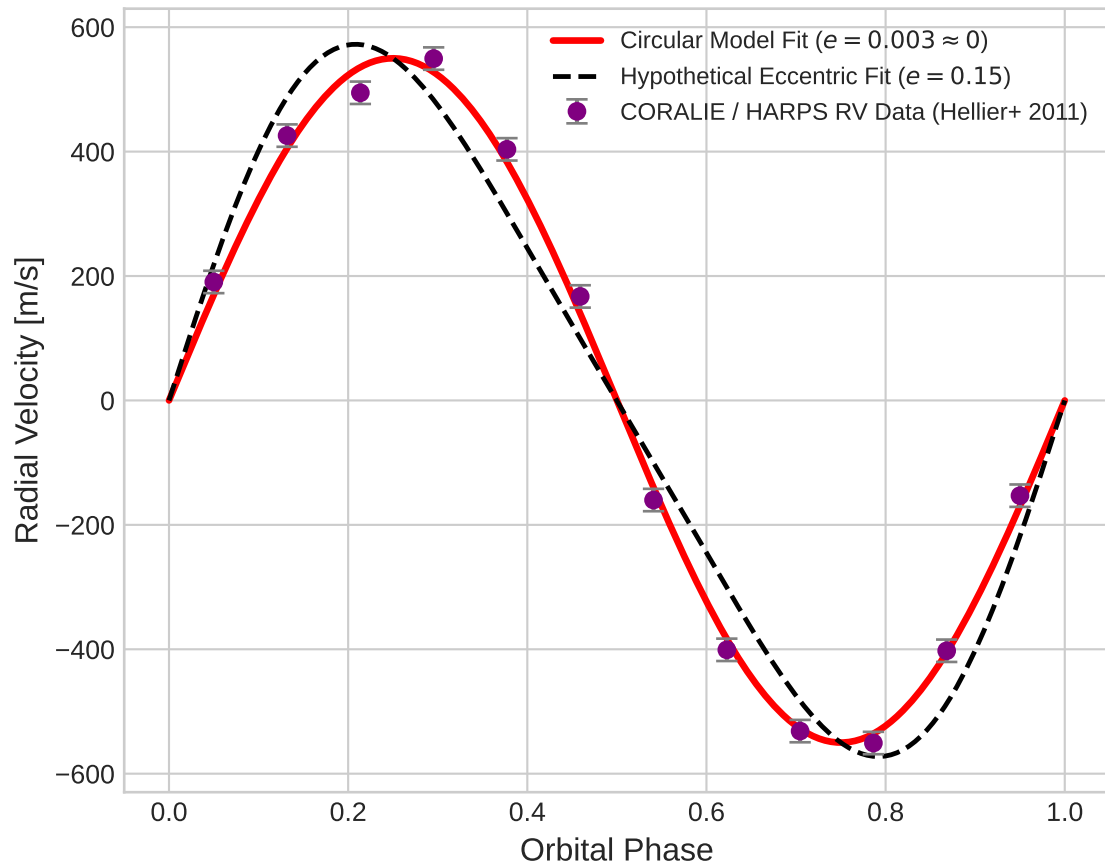
WASP-43 Radial Velocity Circular Orbit Fit
