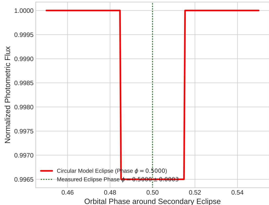
Secondary Eclipse Timing: e \cos \omega = 0.0000
