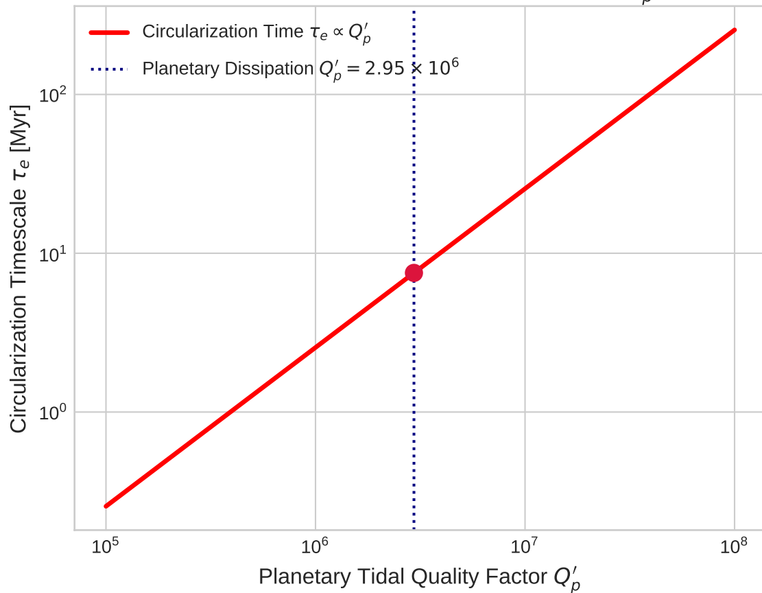
Model Choice: Timescale vs Planetary Q'_p
