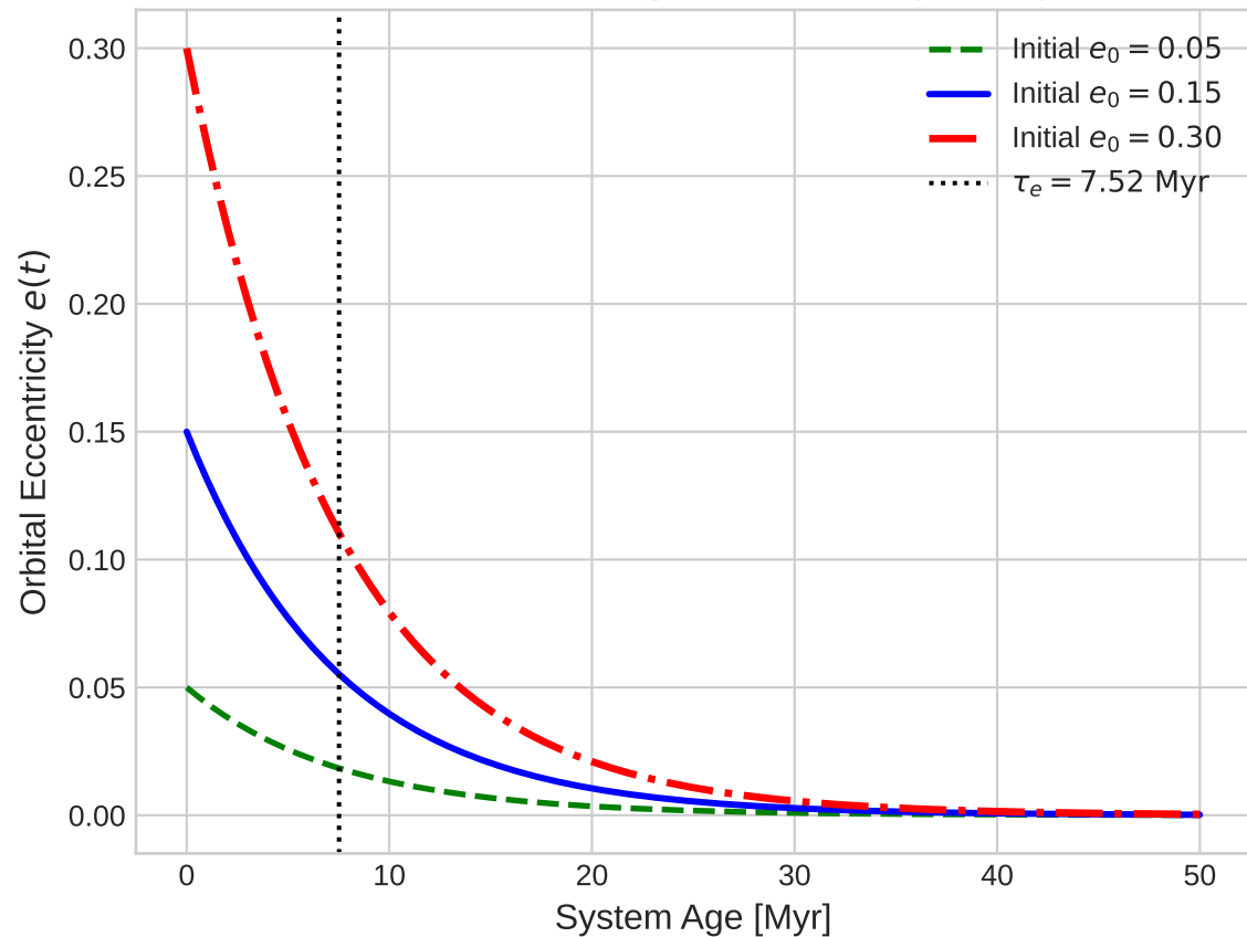
Model Choice: Rapid Eccentricity Decay
