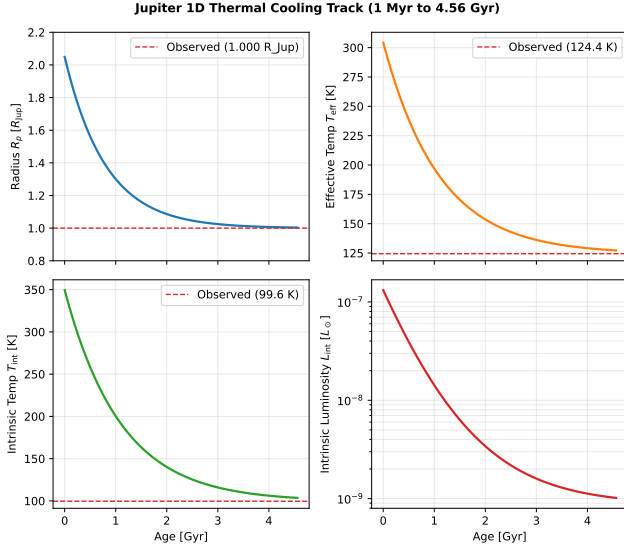
Figure 1: Scenario 1: 4-Panel diagnostic thermal cooling track for Jupiter ( M_p = 1.00 M_{\text{Jup}} , M_c = 12.0 M_{\oplus} , a = 5.204 AU) from t = 1 Myr to 4.56 Gyr.
